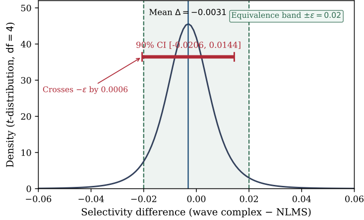
Figure 6: Two one-sided t -test (TOST at \alpha = 0.05 , 90% CI) on retrieval selectivity between wave complex and normalized delta ( \varepsilon = 0.02 , n = 5 seeds). Mean difference: -0.0031 ; 90% CI: [-0.0206, 0.0144] . The confidence interval crosses -\varepsilon by 0.0006.
