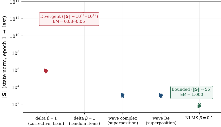
Figure 3: State-norm evolution (log scale, epoch 1 to final epoch). Corrective delta with \beta = 1 diverges ( \|\mathbf{S}\| \sim 10^{11}-10^{12} , \text{EM} \approx 0.03-0.05 ). Superposition writes (wave complex, wave Re) remain bounded. Normalized-key delta with \beta = 0.1 maintains bounded state norm and achieves \text{EM} = 1.000 .
