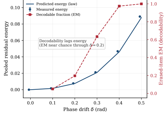
Figure 5: Key/Re cell at D = 128 : pooled residual energy versus erased-item EM (ridge decodability). Erased-item EM is undefined at \delta = 0 (residuals are null-guarded) and stays within a few times chance through \delta \approx 0.2 , rising clearly by \delta = 0.4 ; pooled energy grows smoothly throughout.
