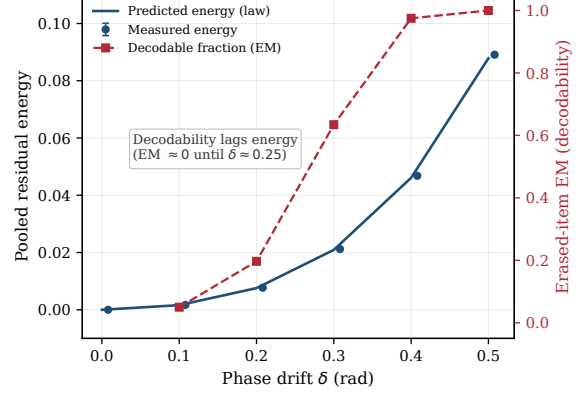
Figure 5: Key/Re cell at D = 128 : pooled residual energy versus erased-item EM (ridge decodability). Decodability remains near zero until \delta \approx 0.25 and rises sharply by \delta \approx 0.4 , whereas energy grows smoothly throughout.
