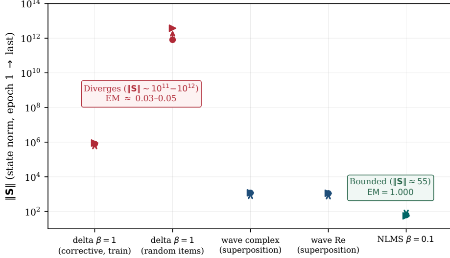
Figure 3: State-norm evolution (log scale, epoch 1 to final epoch). Corrective delta with \beta = 1 diverges ( \|S\| \sim 10^{11}-10^{12} ) ( EM \approx 0.03-0.05 ). Superposition writes (wave complex, wave Re) remain bounded. Normalized-key delta with \beta = 0.1 maintains a bounded state norm and reaches EM = 1.000 .
