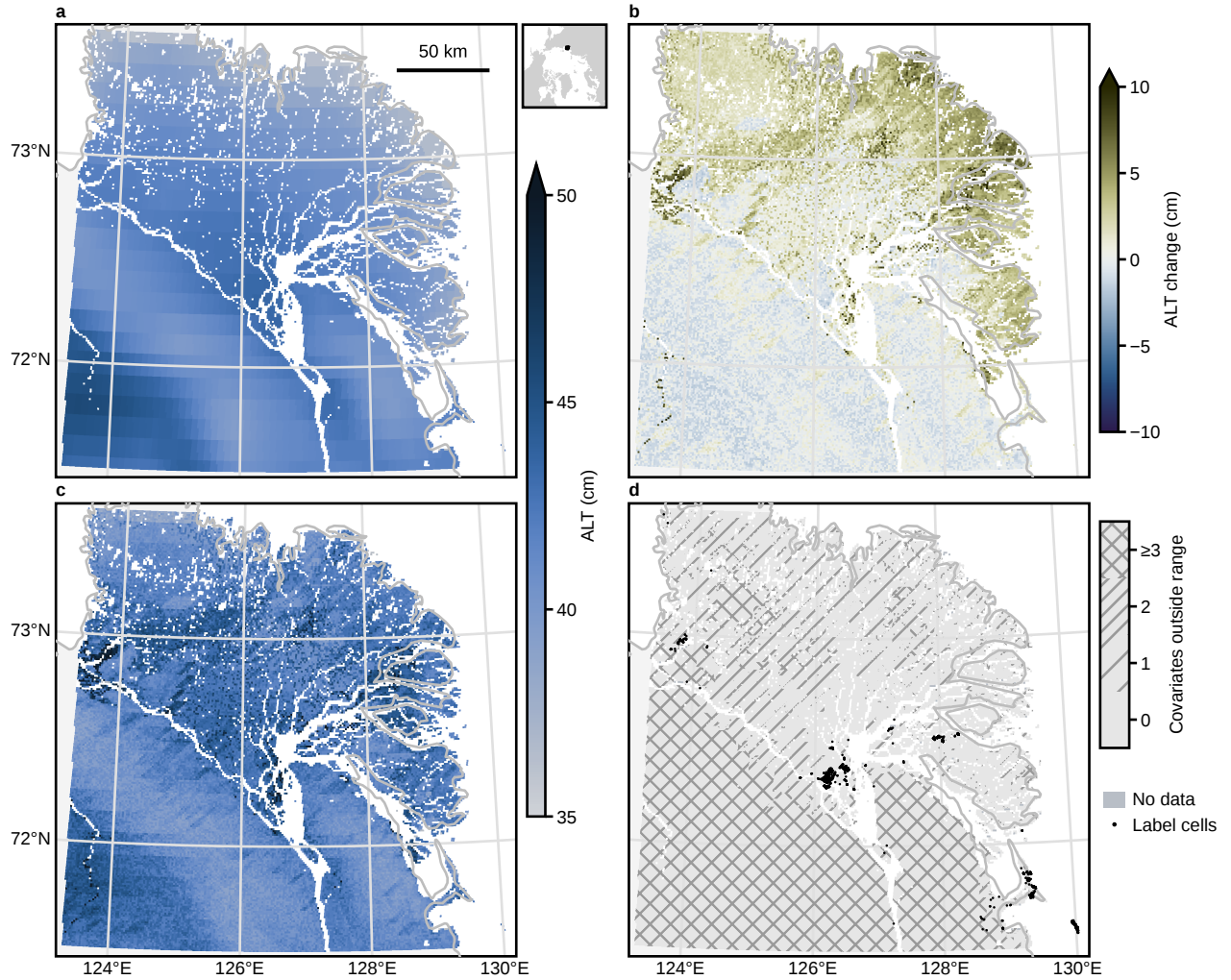
Supplementary Fig. S11 Active-layer thickness (ALT) of the Lena River Delta at 1 km display resolution: recalibrated Stefan model, residual machine-learning correction and final map. a, Recalibrated Stefan ALT, E \cdot \sqrt{TDD} with E = 1.435 (least squares on all 3,037 Lena label cells, shrunk towards the source coefficient 1.619). b, Residual ML correction 0.25 \cdot g (final minus recalibrated Stefan; positive, deeper), where g is a CatBoost residual model (mean of two seeds) fitted to residuals of source-region cells beyond a 100 km buffer and of the Lena labels. c, Final ALT, a plus b. a and c share one colour scale (35–50 cm, 1st–99th percentile of both maps). d, Number of covariates outside the 0.5–99.5 percentile range of the training rows of c (source cells and Lena labels), with label cells as dots; 84% of mapped cells have at least one, mostly ERA5-Land coldest-month temperature, mean annual air temperature and freezing index. Relative to source cells alone, all have three or more. The 90% prediction interval of c is \pm 25.4 cm everywhere (constant-width split conformal on 0.5^\circ block five-fold cross-validation residuals within the Lena labels; cross-validated RMSE 20.8 cm, recalibrated Stefan 21.5 cm). Its nominal coverage is an average over cells similar to the labels and is not guaranteed in hatched cells, so the width is not mapped. The 1 km grid is a display resolution: air thawing index and climate covariates come from ERA5-Land ( 0.1^\circ , about 3 \times 11 km here), soil covariates from SoilGrids windows at about 5 km, and the residual correction acts mainly at the climate-grid scale (main text, Fig. 7c); the horizontal bands in a follow ERA5-Land rows. Cells are drawn as their native 0.009^\circ rectangles. Grid: 71.5\text{--}73.6^\circ N, 123.3\text{--}130.1^\circ E; 38,086 mapped cells. White, sea or water (Global Surface Water occurrence of at least 50%); grey, missing CCI ALT. Polar stereographic projection (central meridian 126.7^\circ E, true scale at 70^\circ N); inset, location. Data: ALLena thaw-depth compilation (Veremeeva et al. 2025, PANGAEA); ERA5-Land (Copernicus C3S); SoilGrids 2.0 (ISRIC); Copernicus DEM GLO-30 (ESA, AWS Open Data); ESA CCI Permafrost v4.0; JRC Global Surface Water; Natural Earth 10 m; Cartopy 0.23.
