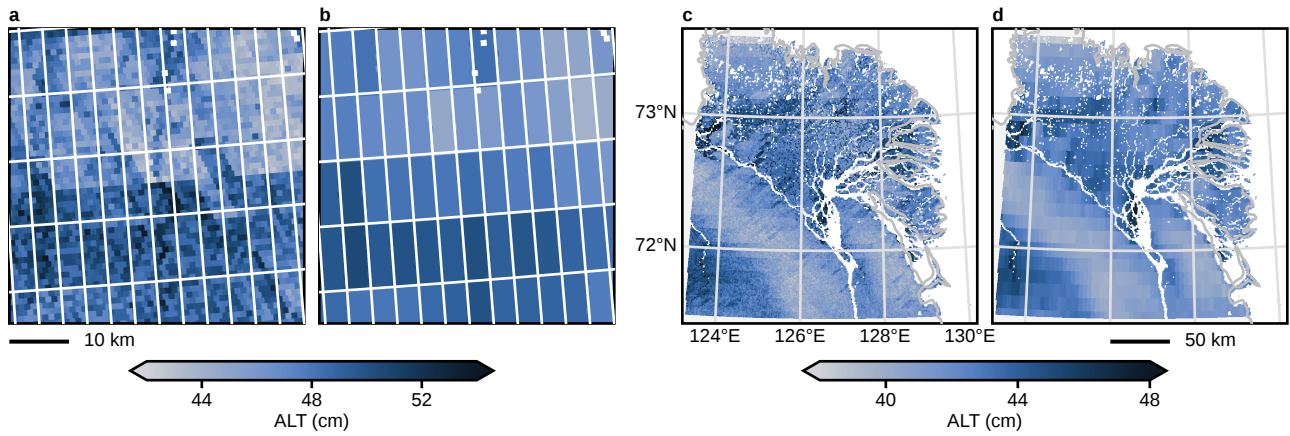
Supplementary Fig. S12 The same residual ML ALT map at its 1 km cells and as ERA5-Land 0.1° cell means. a, b, Alaska, 50 × 50 km around the 0.5° block with the most label cells (69.1° N, 148.8° W; 2,892 cells); white lines, ERA5-Land 0.1° cell boundaries. c, d, Lena Delta, full grid. a and c show the 1 km cells; b and d colour each cell with the mean of the mapped cells in its ERA5-Land 0.1° cell (boundaries at grid point \pm 0.05^\circ ). All cells are drawn as their native 0.009° rectangles without resampling. One colour scale per region from the 1st–99th percentile of both panels (Alaska 42–54 cm, Lena Delta 38–48 cm), narrower than in Supplementary Figs S10 and S11 so that within-cell detail is visible. The 0.1° cell means explain 97% (Alaska, whole domain) and 61% (Lena Delta) of the variance of the 1 km map; the standard deviation of the 1 km values around their 0.1° cell mean is 1.8 cm in Alaska (total 9.5 cm) and 1.1 cm in the Lena Delta (total 1.8 cm). The 1 km map is a display resolution; its information resolution is bound to the climate input (ERA5-Land, about 10 km) and the soil input (SoilGrids, about 5 km). Within-cell detail comes from the terrain (Copernicus DEM 30 m windows) and CCI ALT inputs. Projections as in Supplementary Figs S10 and S11 (NAD83 Alaska Albers; polar stereographic, central meridian 126.7° E). Data as in Supplementary Figs S10 and S11; Cartopy 0.23.
