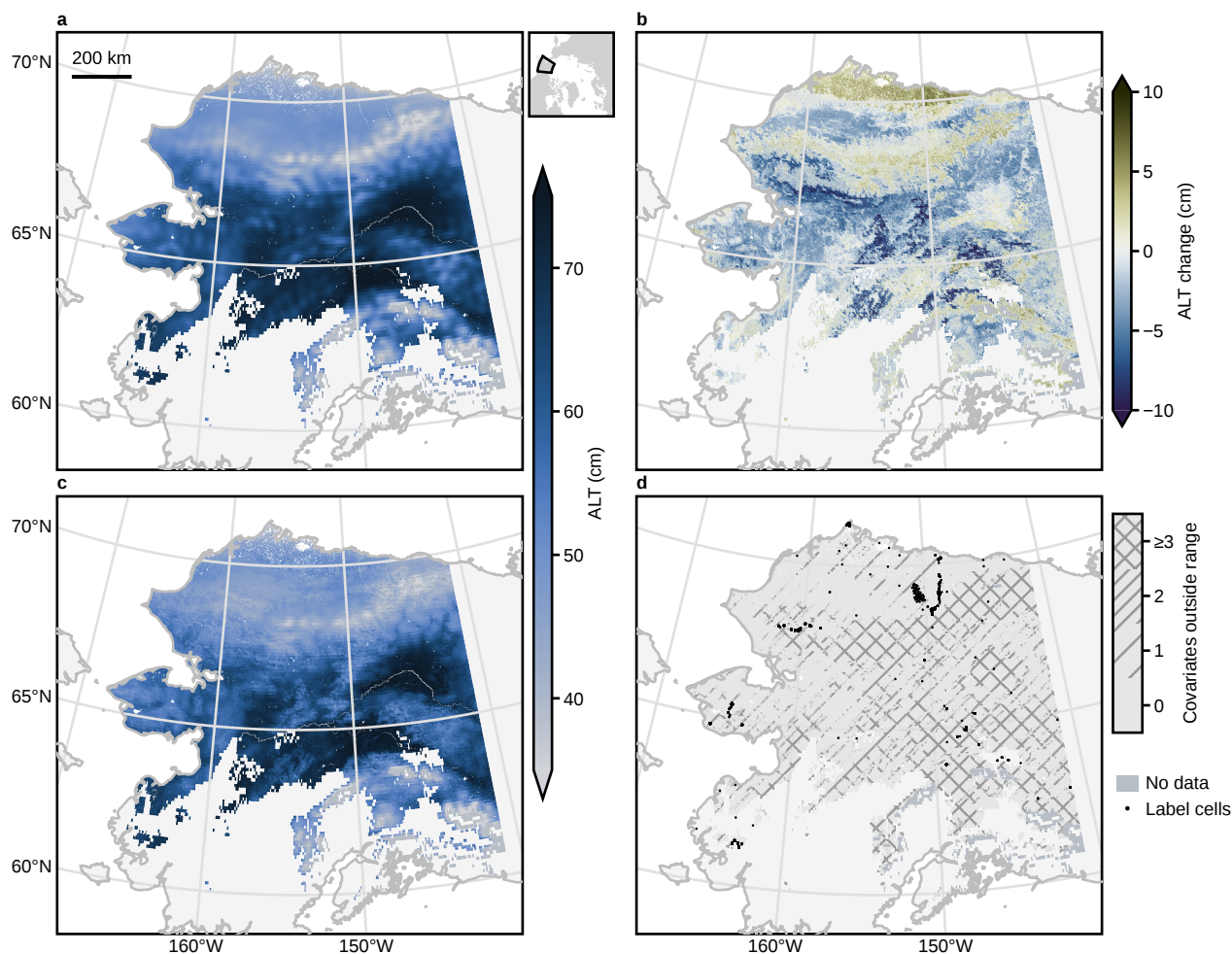
Supplementary Fig. S10 Active-layer thickness (ALT) of the Alaskan permafrost zone at 1 km display resolution: recalibrated Stefan model, residual machine-learning correction and final map. a, Recalibrated Stefan ALT, E \cdot \sqrt{TDD} with E = 1.617 (least squares on all 13,606 label cells, shrunk towards the source coefficient). b, Residual ML correction \lambda \cdot g (final minus recalibrated Stefan; positive, deeper), where g is a CatBoost residual model on 25 covariates (mean of two seeds) and \lambda = 0.5 was selected from 0.25, 0.5, 1.0 by 0.5^\circ block five-fold cross-validation. c, Final ALT, a plus b. a and c share one colour scale (35–75 cm, 1st–99th percentile of both maps). d, Number of covariates outside the 0.5–99.5 percentile range of the training labels (hatching density), with label cells as dots; 73% of mapped cells have at least one, mostly terrain roughness, slope and topographic position. The 90% prediction interval of c is \pm 20.2 cm everywhere (constant-width split conformal on block cross-validation residuals; cross-validated RMSE 13.8 cm, recalibrated Stefan 14.3 cm; lower bound truncated at 0 cm in 5,384 cells). Its nominal coverage is an average over cells similar to the labels and is not guaranteed in hatched cells, so the width is not mapped. The 1 km grid is a display resolution: air thawing index and climate covariates come from ERA5-Land ( 0.1^\circ , about 4\text{--}6 \times 11 km here), soil covariates from SoilGrids windows at about 5 km, and the residual correction acts mainly between climate-grid cells (main text, Fig. 7c). Cells are drawn as their native 0.009^\circ rectangles. Domain: land (Natural Earth 10 m) with ESA CCI permafrost fraction of at least 50% (1997–2021 mean), 59\text{--}71.5^\circ N, 168\text{--}141^\circ W; 858,517 of 899,633 cells mapped. White, sea or water (Global Surface Water occurrence of at least 50%); grey, missing CCI ALT or soil thaw index. NAD83 Alaska Albers (EPSG:3338); inset, location. Data: ABoVE ALT v2 (Moore et al. 2025, ORNL DAAC) and GTN-P/CALM (Streletskiy et al. 2025) labels; ERA5-Land (Copernicus C3S); SoilGrids 2.0 (ISRIC); Copernicus DEM GLO-30 (ESA, AWS Open Data); ESA CCI Permafrost v4.0; JRC Global Surface Water; Natural Earth; Cartopy 0.23.
