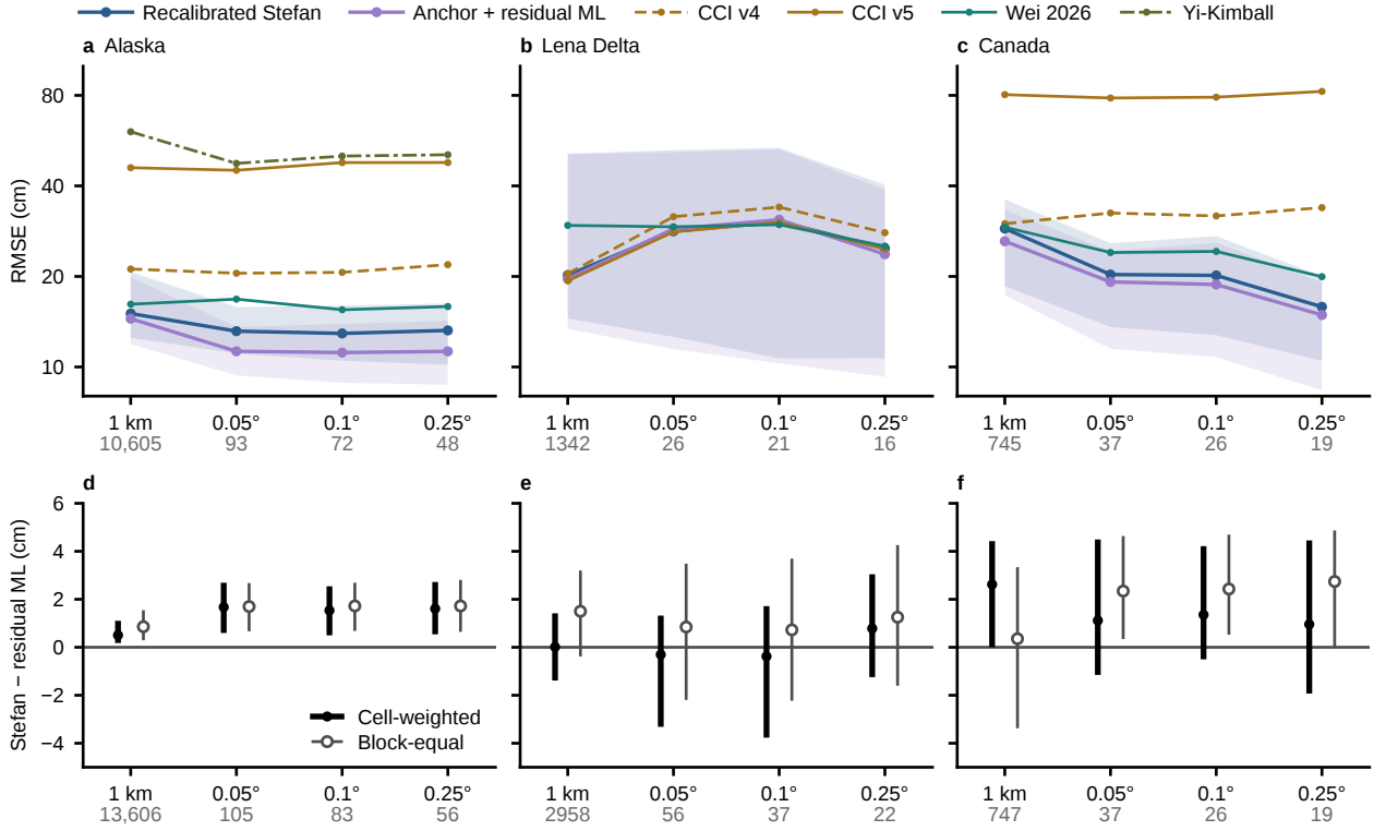
Supplementary Fig. S15 Prediction error of the recalibrated Stefan model, the residual ML model and four ALT products after aggregation to larger grid cells. Model values are within-region out-of-block predictions from 0.5^\circ block five-fold cross-validation; the Stefan coefficient is refitted on the training folds, and \lambda of the residual model is selected by an inner block cross-validation within the training folds. Product values are period means at the label cells: CCI v4 (1997–2021), CCI v5 (1997–2023), Wei 2026 (2000–2024) and, for Alaska, Yi-Kimball (2001–2015). Labels and predictions are averaged in grid cells of 0.05^\circ , 0.1^\circ and 0.25^\circ whose boundaries follow the ERA5-Land cells ( 0.1^\circ = \text{ERA5-Land cell} ); grid cells with fewer than three label cells are dropped; 1 km denotes single label cells. Grey numbers, grid cells per size. a–c, Cell-weighted RMSE (logarithmic axis) on the cells where all shown values exist (Alaska 10,605 cells in 60 blocks, Lena Delta 1,342 in 15, Canada 745 in 34); bands, 95% block bootstrap intervals for the two models (1,000 resamples of 0.5^\circ blocks). d–f, RMSE of the recalibrated Stefan model minus RMSE of the residual ML model on all label cells with model values (Alaska 13,606, Lena Delta 2,958, Canada 747), cell-weighted (filled) and block-equal (open) with 95% block bootstrap intervals. In Alaska the cell-weighted difference is 0.50 cm (0.18 to 1.10) for single cells and 1.54 to 1.67 cm (lower bounds 0.50 to 0.60) at 0.05^\circ , 0.1^\circ and 0.25^\circ . In Canada it is 2.62 cm (0.00 to 4.42) for single cells and 0.96 to 1.35 cm at larger sizes, with intervals that include zero. In the Lena Delta all intervals include zero. Removing cells within 5 km of Wei 2026 training sites changes the Alaska differences by at most 0.17 cm (data/processed/xbatch/XK_support_scale/). Products are compared only as RMSE differences at the same grid size.
