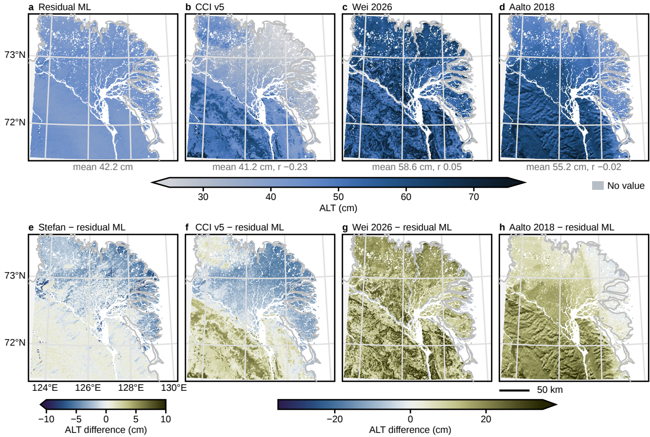
Supplementary Fig. S14 The 1 km Lena Delta ALT map compared with three ALT products and with the recalibrated Stefan model. a–d, ALT of the residual ML map (a, as in Supplementary Fig. S11) and of CCI v5 (1997–2023 mean, b), Wei 2026 (2000–2024 mean, c) and Aalto 2018 (2000–2014 baseline, d) on one colour scale (25–75 cm, 2nd–98th percentile of all four maps over mapped cells). Grey text, area mean over mapped cells with a product value and Pearson correlation r with the residual ML map. e, Recalibrated Stefan – residual ML on its own scale ( \pm 10 cm, the scale of panel b of Supplementary Figs S10 and S11 with the sign reversed). f–h, Product – residual ML (positive, product deeper) on one scale ( \pm 35 cm, 98th percentile of the absolute differences of f–h). Products are read at the 1 km cell centres (nearest pixel, period mean). Mean differences are -0.9 cm (CCI v5), +16.5 (Wei 2026, 94% of cells with values), +13.0 (Aalto 2018) and -1.1 cm (Stefan). CCI v5 is shallower than the map in the northern and eastern delta and deeper in the south-western part of the grid; Wei 2026 and Aalto 2018 are deeper over most of the grid. These maps carry no accuracy statement; accuracy is compared only at label cells. The 1 km map is a display resolution; its information resolution is bound to the climate input (ERA5-Land, about 10 km) and the soil input (SoilGrids, about 5 km). Grey cells, no product value. Polar stereographic projection (central meridian 126.7^\circ E, true scale at 70^\circ N). Data: CCI v5 (ESA CCI Permafrost, CEDA); Wei et al. 2026 (Zenodo 21667583, CC BY 4.0); Aalto et al. 2018 (Zenodo 5003804, CC0); covariates and labels as in Supplementary Fig. S11; Natural Earth 10 m; Cartopy 0.23.
