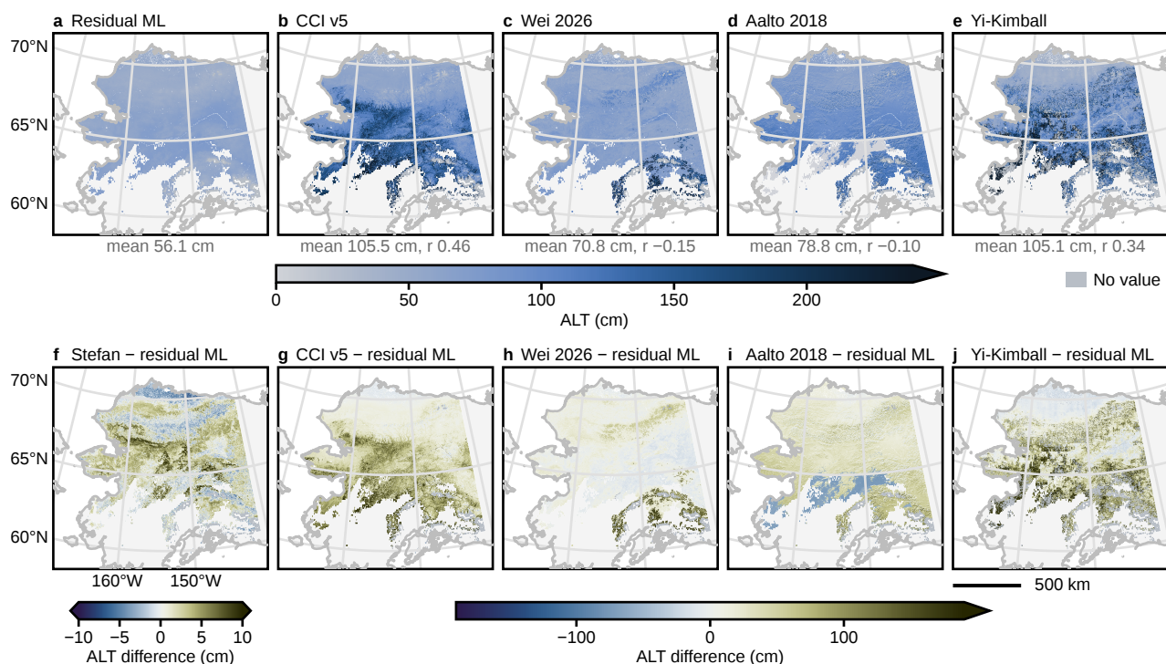
Supplementary Fig. S13 The 1 km Alaska ALT map compared with four ALT products and with the recalibrated Stefan model. a–e, ALT of the residual ML map (a, as in Supplementary Fig. S10) and of CCI v5 (1997–2023 mean, b), Wei 2026 (2000–2024 mean, c), Aalto 2018 (2000–2014 baseline, d) and Yi-Kimball (2001–2015 mean, e) on one colour scale (0–240 cm, 2nd–98th percentile of all five maps over mapped cells). Grey text, area mean over mapped cells with a product value and Pearson correlation r with the residual ML map. f, Recalibrated Stefan – residual ML on its own scale ( \pm 10 cm, the scale of panel b of Supplementary Figs S10 and S11 with the sign reversed). g–j, Product – residual ML (positive, product deeper) on one scale ( \pm 190 cm, 98th percentile of the absolute differences of g–j). Products are read at the 1 km cell centres (nearest pixel, period mean). Mean differences are +49.4 cm (CCI v5), +14.7 (Wei 2026), +22.6 (Aalto 2018), +49.3 (Yi-Kimball) and +1.4 cm (Stefan). Large differences with CCI v5 and Yi-Kimball are widespread in Interior Alaska; the largest differences with Wei 2026 lie at about 61–63° N, 141–150° W; Aalto 2018 is shallower than the map at about 62–64° N west of 148° W. These maps carry no accuracy statement; accuracy is compared only at label cells (Supplementary Table S13 and Supplementary Fig. S15). The 1 km map is a display resolution; its information resolution is bound to the climate input (ERA5-Land, about 10 km) and the soil input (SoilGrids, about 5 km). Grey cells, no product value (Yi-Kimball covers 86% of mapped cells). NAD83 Alaska Albers (EPSG:3338). Data: CCI v5 (ESA CCI Permafrost, CEDA, doi:10.5285/a6fbdd8ee5b472c8e84e55f746c1704); Wei et al. 2026 (Zenodo 21667583, CC BY 4.0); Aalto et al. 2018 (Zenodo 5003804, CC0); Yi and Kimball (ORNL DAAC 1760); covariates and labels as in Supplementary Fig. S10; Natural Earth 10 m; Cartopy 0.23.
