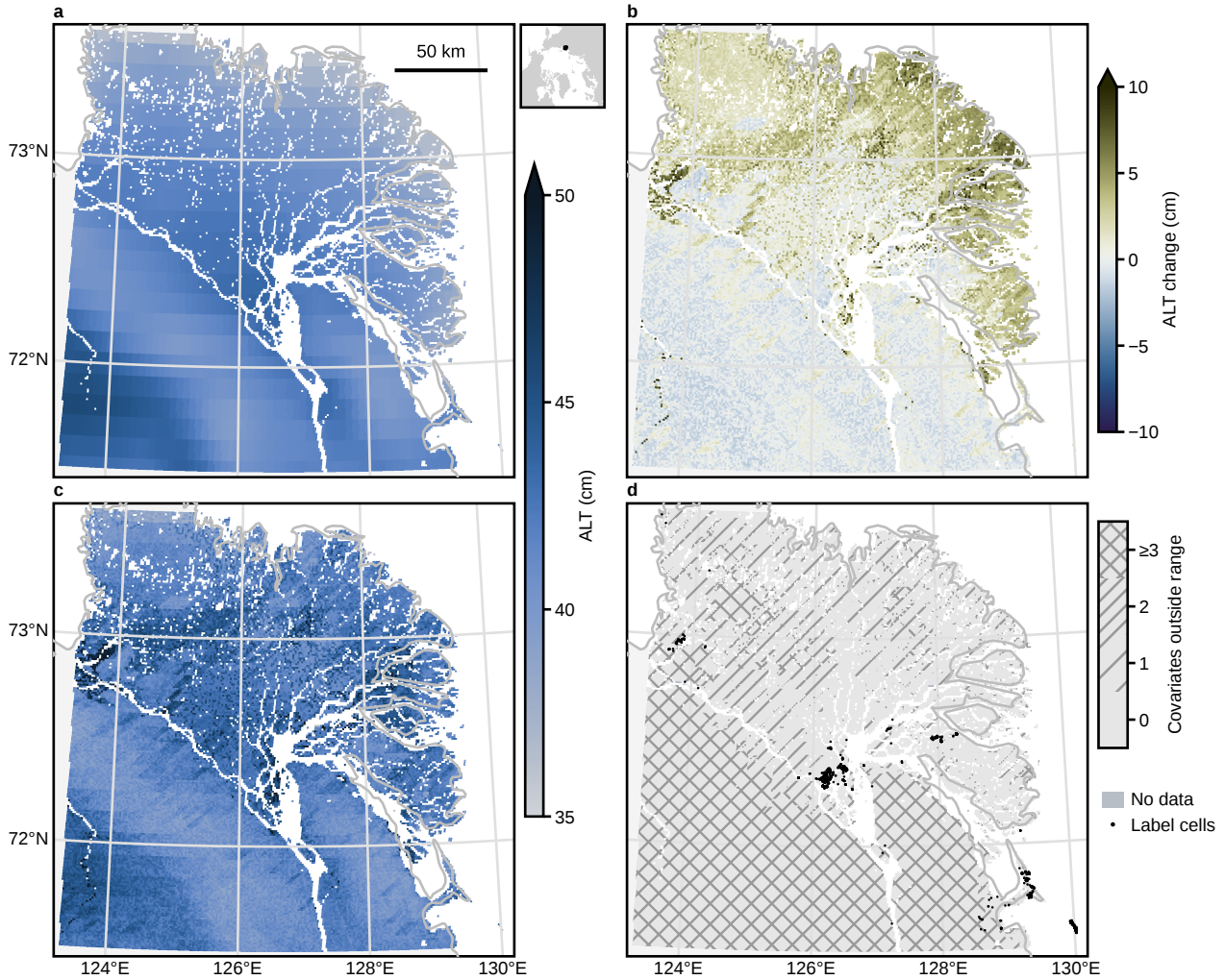
Supplementary Fig. S11 Active-layer thickness (ALT) of the Lena River Delta at 1 km display resolution: recalibrated Stefan model, residual machine-learning correction and final map. a, Recalibrated Stefan ALT, E \cdot \sqrt{TDD} with E = 1.435 (least squares on all 3,037 Lena label cells, shrunk towards the source coefficient 1.619). b, Residual ML correction 0.25 \cdot g (final minus recalibrated Stefan; positive, deeper), where g is a CatBoost residual model (mean of two seeds) fitted to residuals of source-region cells beyond a 100 km buffer and of the Lena labels. c, Final ALT, a plus b. a and c share one colour scale (35–50 cm, 1st–99th percentile of both maps). d, Number of covariates outside the 0.5–99.5 percentile range of the training rows of c (source cells and Lena labels), with label cells as dots; 84% of mapped cells have at least one, mostly ERA5-Land coldest-month temperature, mean annual air temperature and freezing index. Relative to source cells alone, all have three or more. The 90% prediction interval of c is \pm 25.4 cm everywhere (constant-width split conformal on 0.5^\circ block five-fold cross-validation residuals within the Lena labels; cross-validated RMSE 20.8 cm, recalibrated Stefan 21.5 cm). Its nominal coverage is an average over cells similar to the labels and is not guaranteed in hatched cells, so the width is not mapped. The 1 km grid is a display resolution: air thawing index and climate covariates come from ERA5-Land ( 0.1^\circ , about 3 \times 11 km here), soil covariates from SoilGrids windows at about 5 km, and the residual correction acts mainly at the climate-grid scale (main text, Fig. 7c); the horizontal bands in a follow ERA5-Land rows. Cells are drawn as their native 0.009^\circ rectangles. Grid: 71.5\text{--}73.6^\circ N, 123.3\text{--}130.1^\circ E; 38,086 mapped cells. White, sea or water (Global Surface Water occurrence of at least 50%); grey, missing CCI ALT. Polar stereographic projection (central meridian 126.7^\circ E, true scale at 70^\circ N); inset, location. Data: ALLena thaw-depth compilation (Veremeeva et al. 2025, PANGAEA); ERA5-Land (Copernicus C3S); SoilGrids 2.0 (ISRIC); Copernicus DEM GLO-30 (ESA, AWS Open Data); ESA CCI Permafrost v4.0; JRC Global Surface Water; Natural Earth 10 m; Cartopy 0.23.
