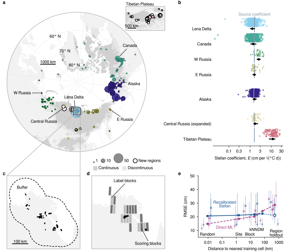
Figure 1. Study regions, Stefan coefficients and evaluation design. (a) Labelled cells of the licence-verified label tables in 0.5^{\circ} blocks; circle area is proportional to the number of 1 km label locations in a block, colour marks the region as in (b) (grey, Greenland, Svalbard and Scandinavia), and New regions marks the regions added after the label tables were fixed (Central Russia, expanded edition; Tibetan Plateau, inset; Table 1). Shading shows continuous (permafrost fraction \geq 90\% ) and discontinuous (50–90%) permafrost (ESA CCI Permafrost fraction v4.0, 1997–2021 mean); rectangle, area of c and d. (b) Stefan coefficient E = \text{ALT}/\sqrt{\text{TDD}} of labelled cells by region (logarithmic axis), where ALT is the active-layer thickness and TDD the ERA5-Land 6 air thawing index ( ^{\circ}\text{C d} , 2015–2020 mean); up to 400 cells per region, median and interquartile range; Source coefficient, the coefficient fitted on the source pool when that region is held out. (c) Region holdout: labelled cells of the Lena Delta and all cells within 100 km (Buffer) are removed from the training data. (d) Split of the same region into label and scoring blocks (one of five splits), with 40 label cells drawn from the label blocks and errors scored only in the scoring blocks. The within-region tests use the same block split without source data and were designed after the transfer results had been inspected. (e) RMSE against median distance from scoring to nearest training cell, from random-cell to region-holdout validation (lines, three-region means; symbols, regions with cell-weighted 95% intervals; open, Stefan with source coefficient). From random-cell to kNNNDM splits, direct-ML RMSE increased by 5.76, 8.17 and 14.20 cm and recalibrated-Stefan RMSE by 0.29, 0.51 and 4.28 cm (Alaska, Lena Delta, Canada; cell-weighted; descriptive, designed after earlier results were viewed). Cells without a verified licence (Canada 38, North Atlantic 19, W Russia 1) are not drawn. Polar stereographic projection (central meridian 127^{\circ} E; scale bar true at 70^{\circ} N), also in c and d; Tibetan Plateau inset, Lambert azimuthal equal-area projection with its own scale bar. Coastlines, Natural Earth 50 m (10 m in c and d); Cartopy 0.23.
