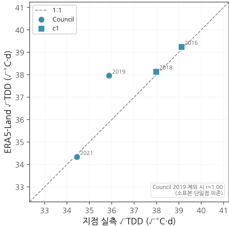
√융해도일 (bias +0.55, r=0.88, n=4)
