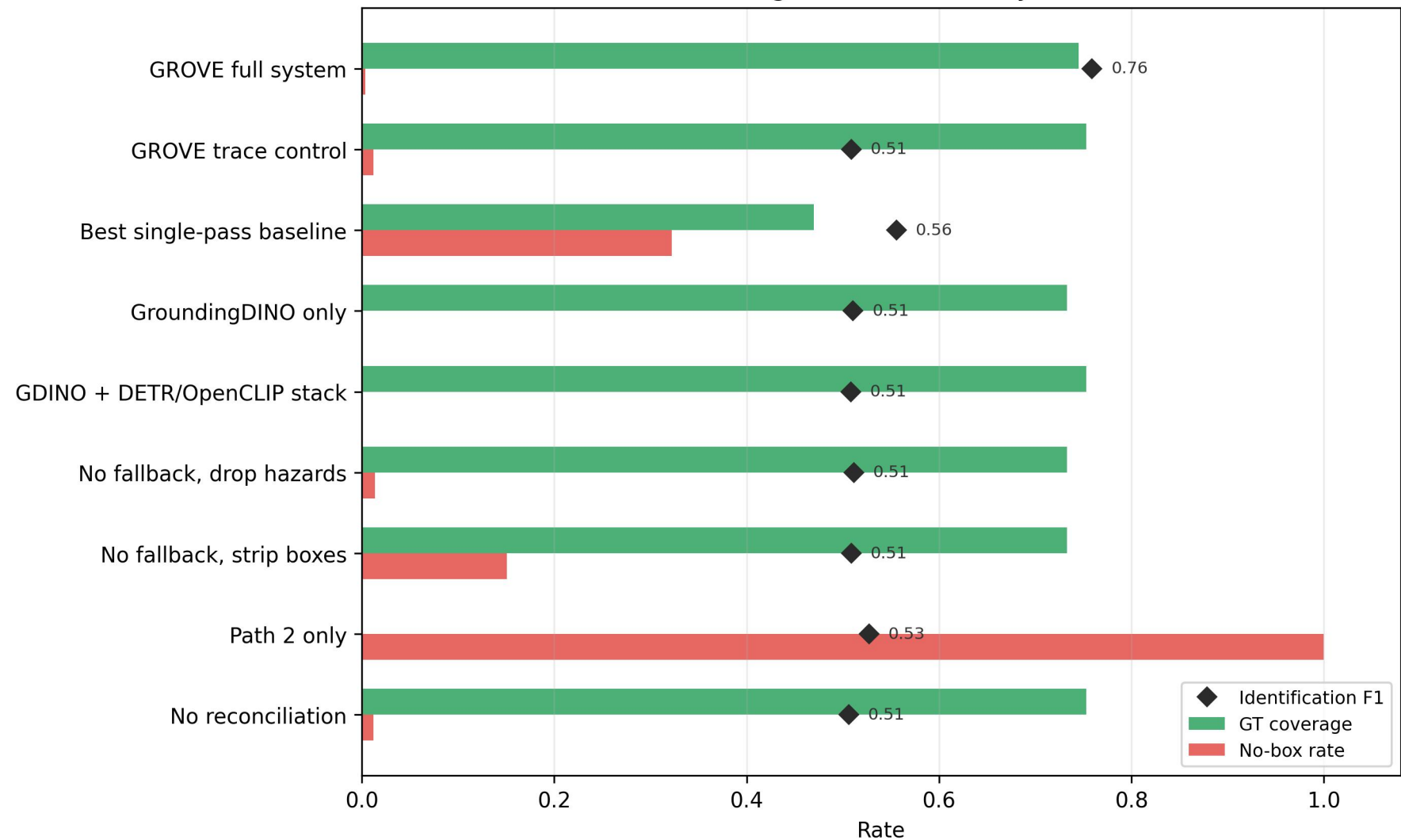
Grounding trade-off across systems
