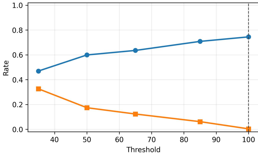
Oversized-box cutoff
