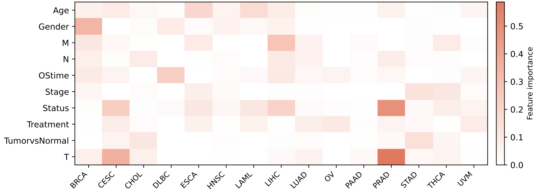
BMP6 Clinical feature importance
