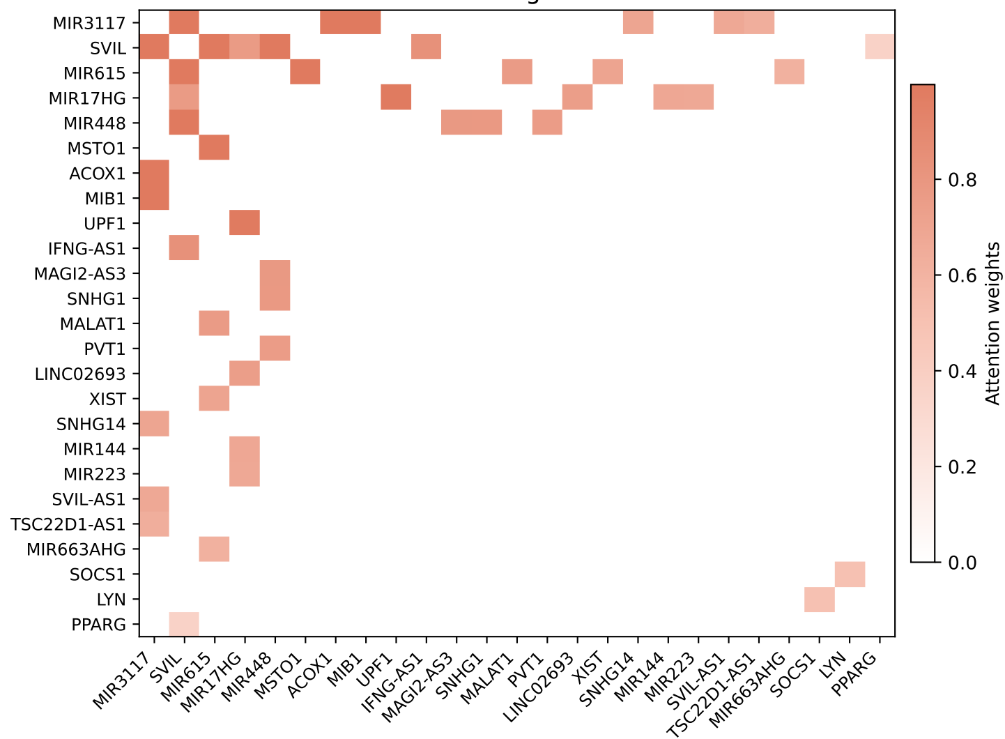
Attention weights of SVIL
