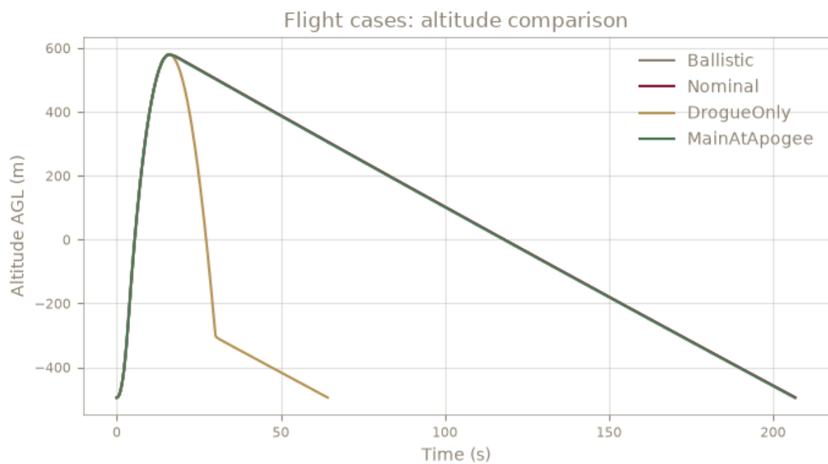
Figure 17. Altitude comparison across the required flight cases.
