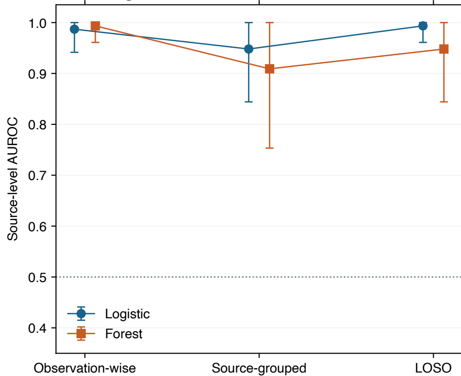
A Ranking
