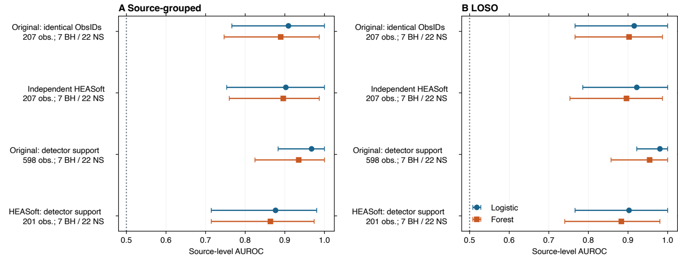
Figure 4: Source-level AUROC under matched-observation and common instrumental-support comparisons, shown separately for source-grouped and LOSO evaluation. The matched-observation comparison uses identical ObsIDs to distinguish processing differences from observation selection as far as the design permits. Common-support rows restrict the representations to the declared instrumental-support criteria but do not constitute exact distributional matching. Error bars are conditional source-bootstrap intervals.
