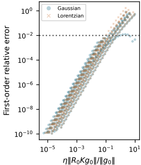
(c) Perturbative organization
