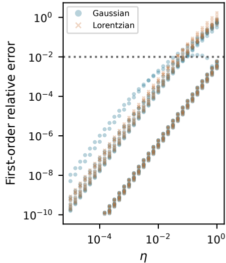
(a) Perturbative organization
