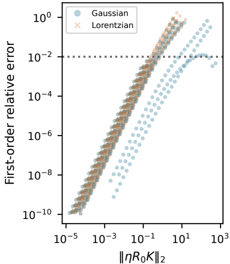
(b) Perturbative organization
