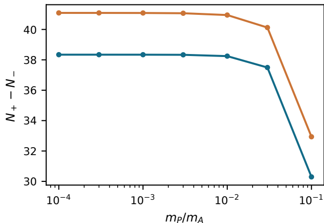
(c) Passive valley displacement
