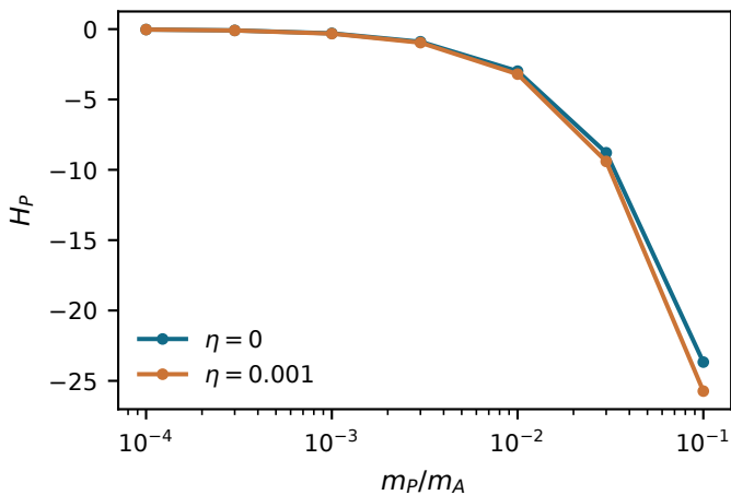
(c) Passive valley displacement
