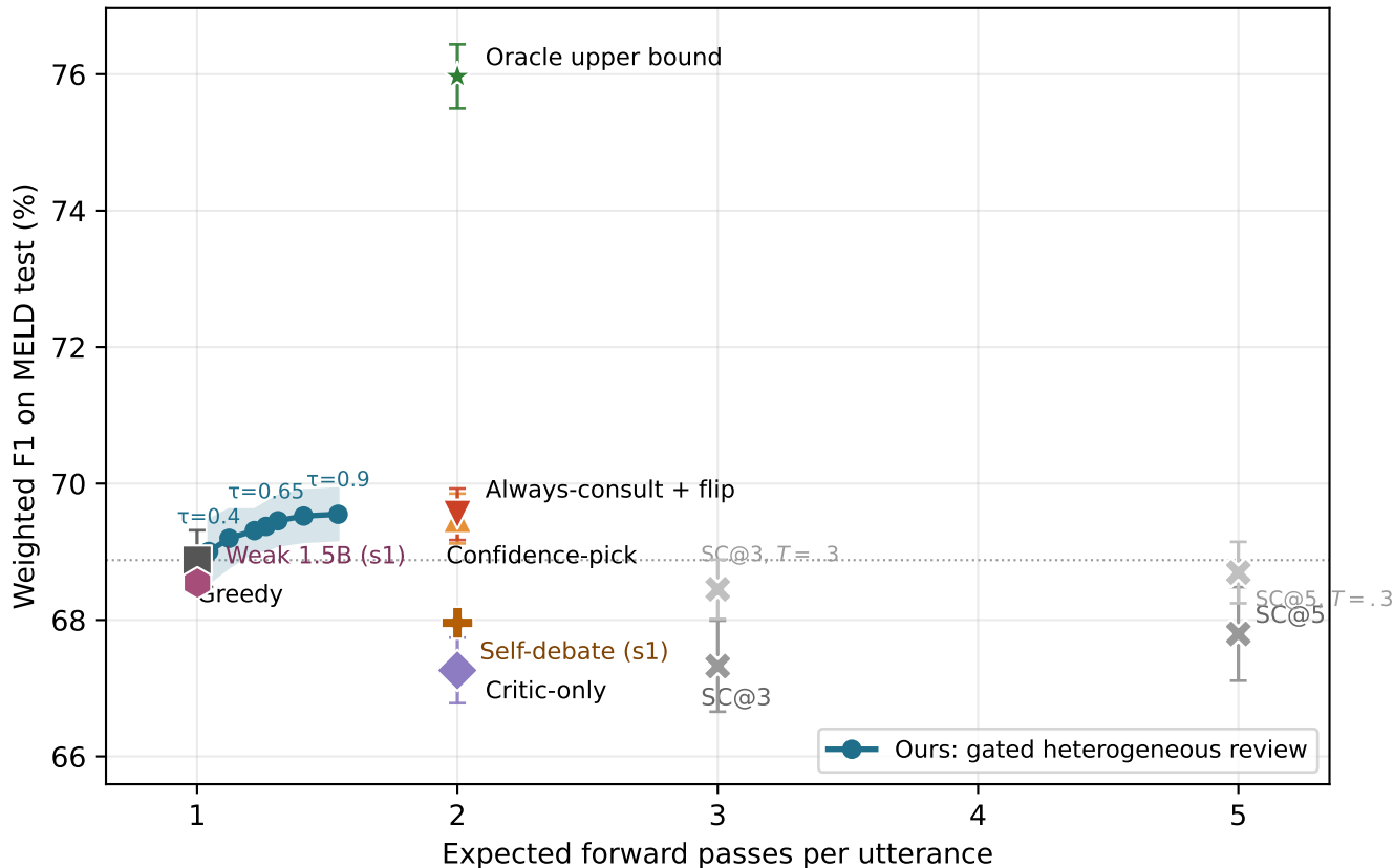
Cost-accuracy Pareto: heterogeneous review vs. baselines (mean \pm sd, 8 seeds)
