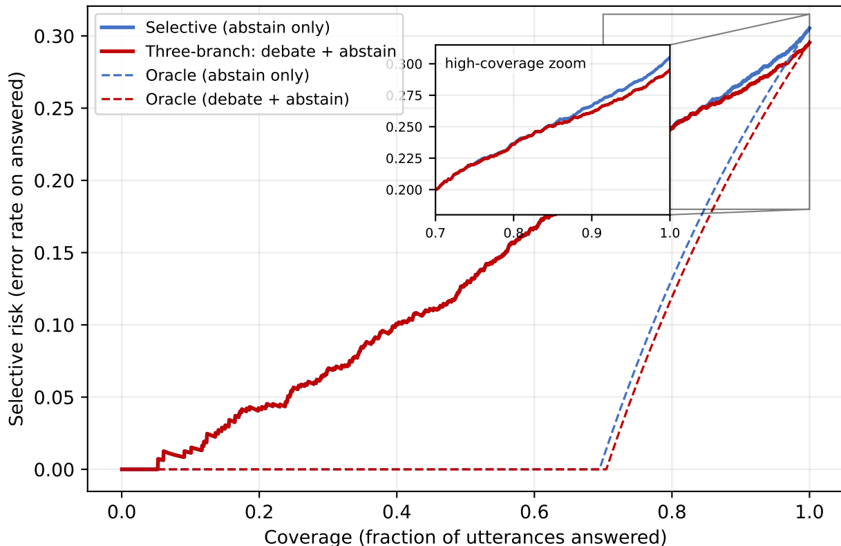
Risk-coverage on MELD test (seed 42, \tau=0.65 )
