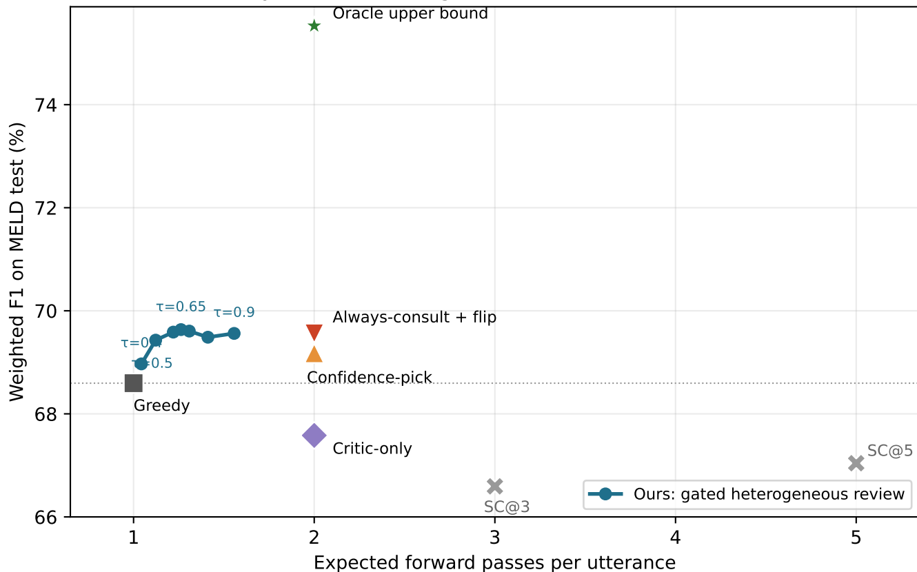
Cost-accuracy Pareto: heterogeneous review vs. baselines (seed 42)
