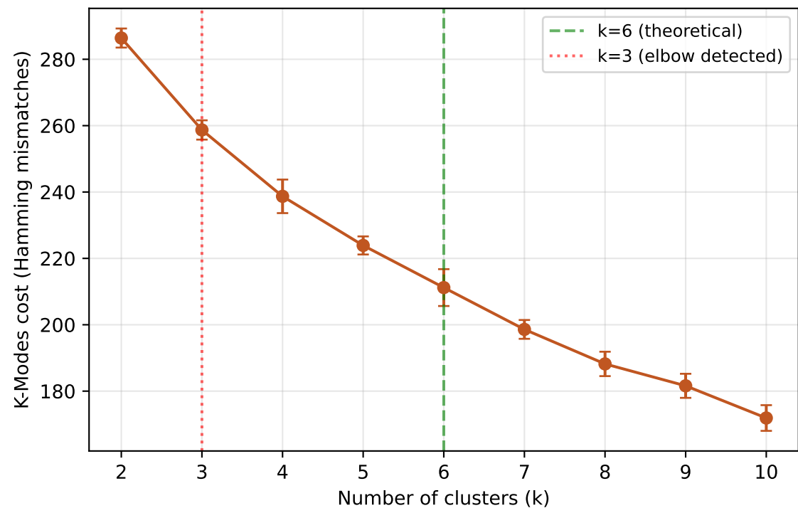
K-Modes Cost Curve
