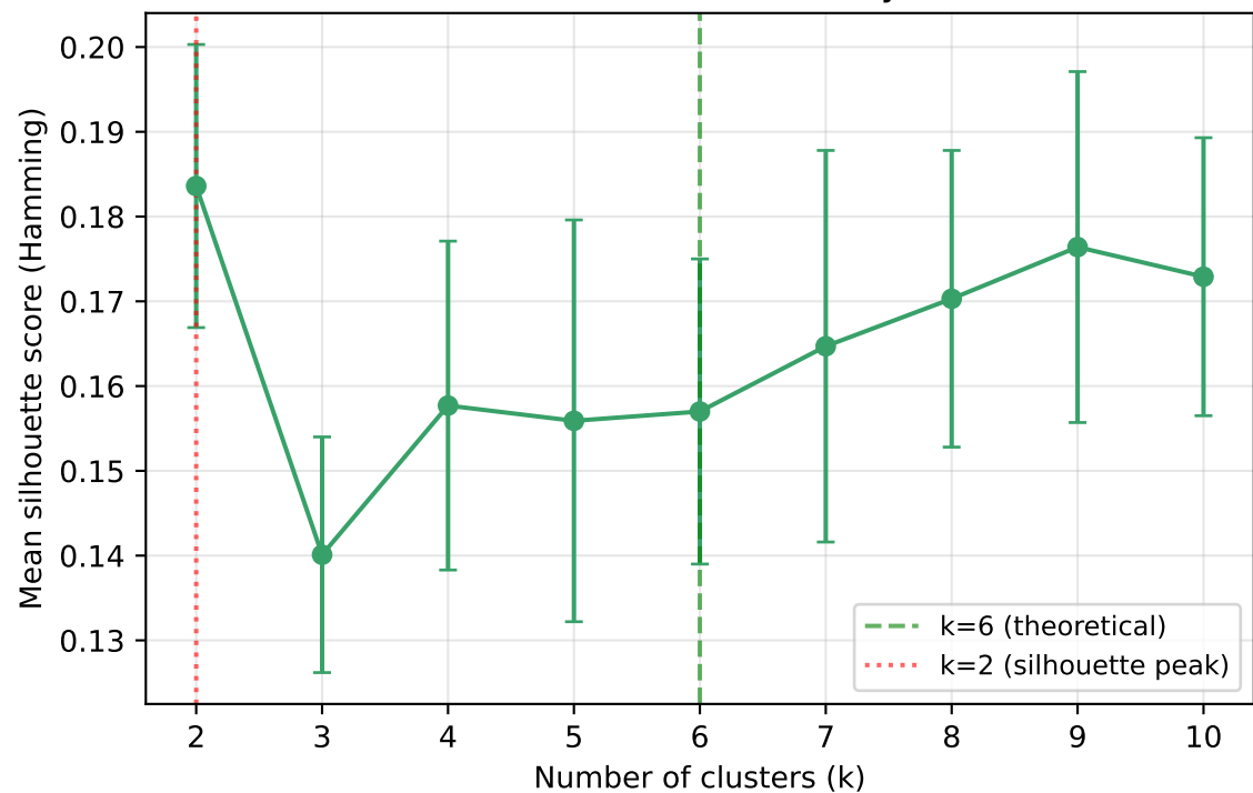
K-Modes Silhouette Analysis
