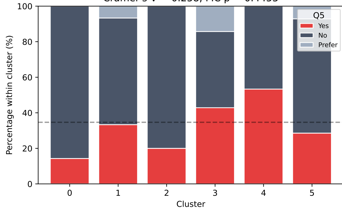
K-Means: Q5 composition per cluster Cramér's V = 0.258, MC p = 0.4453
