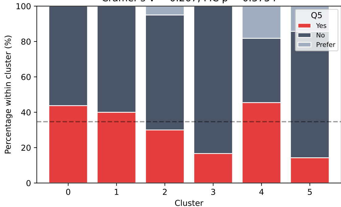
K-Modes: Q5 composition per cluster Cramér's V = 0.267, MC p = 0.3754
