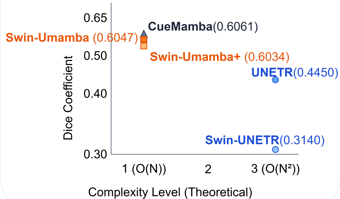
(a) Computational Complexity Level vs. Dice Coefficient
