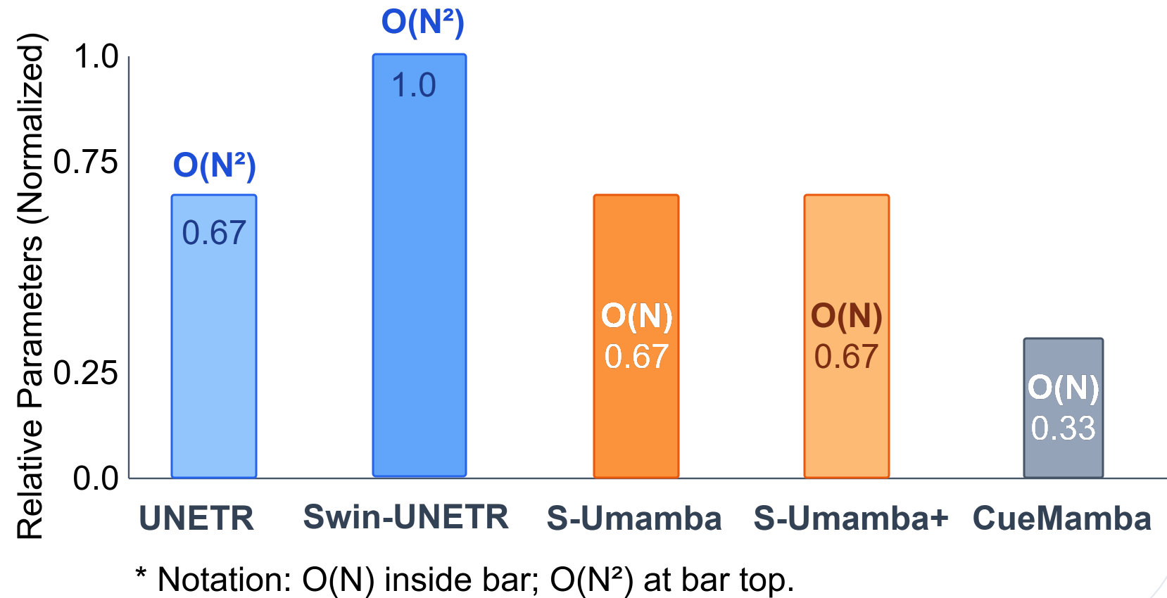
(b) Relative Parameters and Computational Complexity Notation
