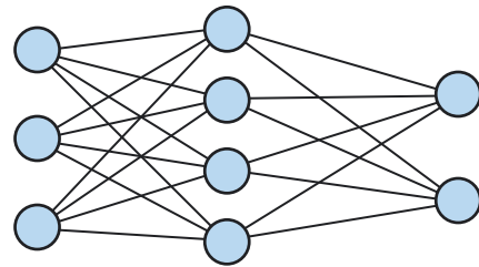
Value Critic
