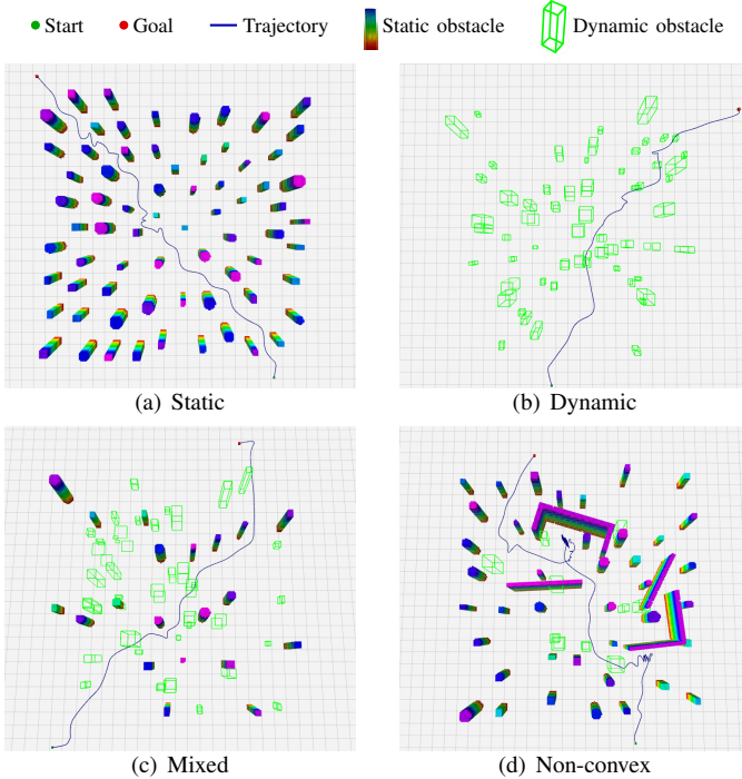
Fig. 4. Representative ForesightNav trajectories in the four simulation environments.
