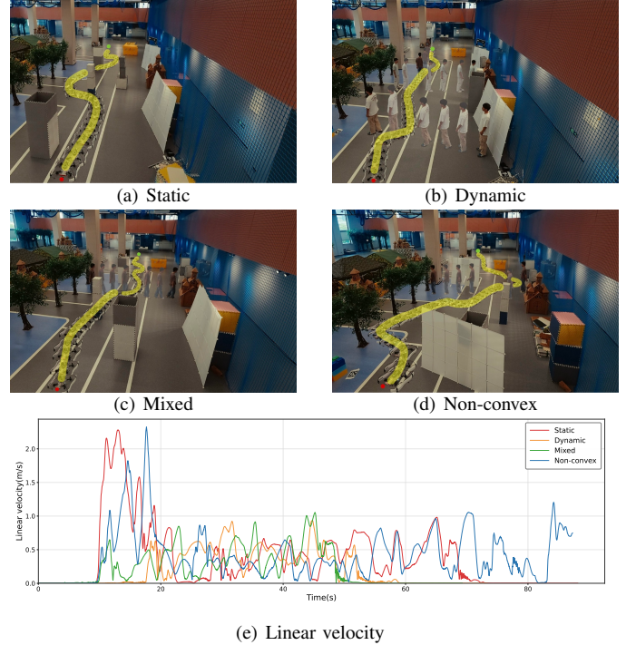
Fig. 6. Zero-shot physical flight tests of ForesightNav in a 28\text{ m} \times 15\text{ m} area. (a) Static obstacles. (b) Dynamic obstacles. (c) Mixed static and dynamic obstacles. (d) Large non-convex structures. (e) UAV linear-velocity profiles in the four environments.
