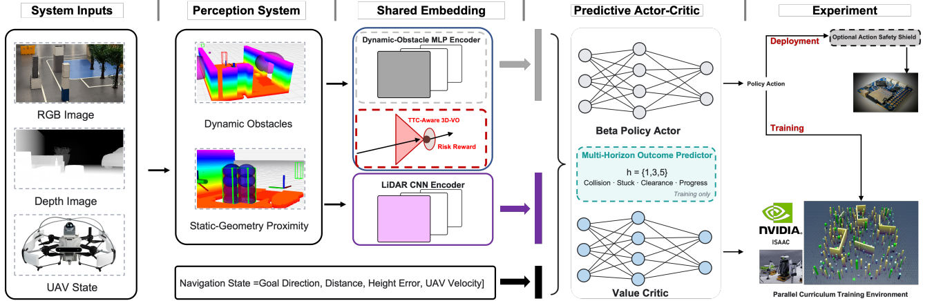
Fig. 1. The proposed ForesightNav framework. The perception system processes RGB-D observations together with the UAV state to form dynamic-obstacle, static-geometry proximity, and navigation representations. Modality-specific MLP and CNN encoders transform these inputs into a shared embedding for the predictive actor-critic. During training, the TTC-aware 3D-VO risk reward and action-conditioned multi-horizon outcome predictor jointly shape policy learning in parallel curriculum environments. During deployment, the outcome predictor is removed, and the Beta-policy actor directly generates velocity actions that can be further refined by an optional safety shield.
