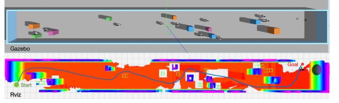
Fig. 5. Safe navigation in a simulated corridor environment. The upper panel shows the Gazebo scene containing static obstacles and moving pedestrians, while the lower panel shows the corresponding environment map and UAV trajectory.
