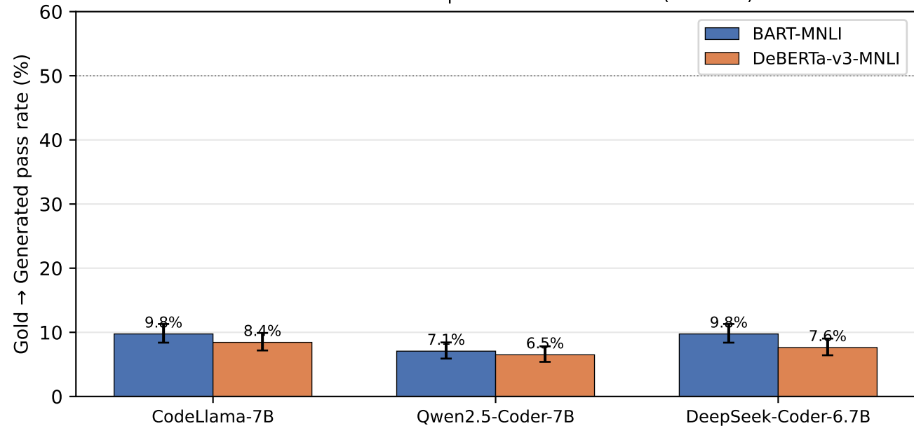
Gold \rightarrow Generated NLI pass rate at \tau = +0.56 (N=1600)
