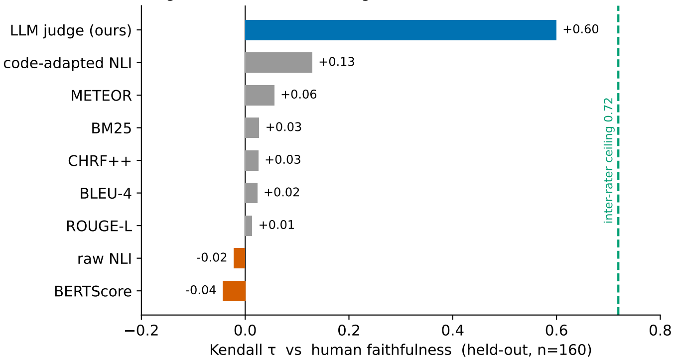
Agreement with human diff-grounded faithfulness labels (held-out)
