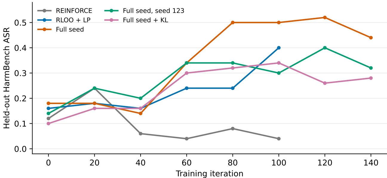
Adversary Training Trajectories
