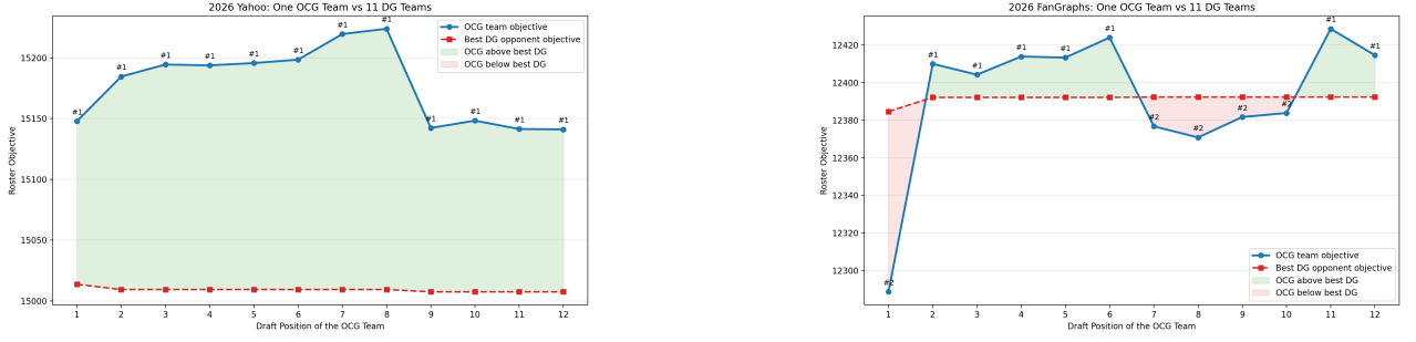
Figure 4: Competitive simulation: one OCG team vs. 11 DG teams across all draft positions. Left: Yahoo; right: FanGraphs. OCG ranks first for Yahoo and either first or second for FanGraphs.
