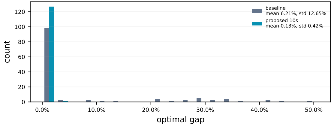
S14 Accepted-Reward Gap Histogram
