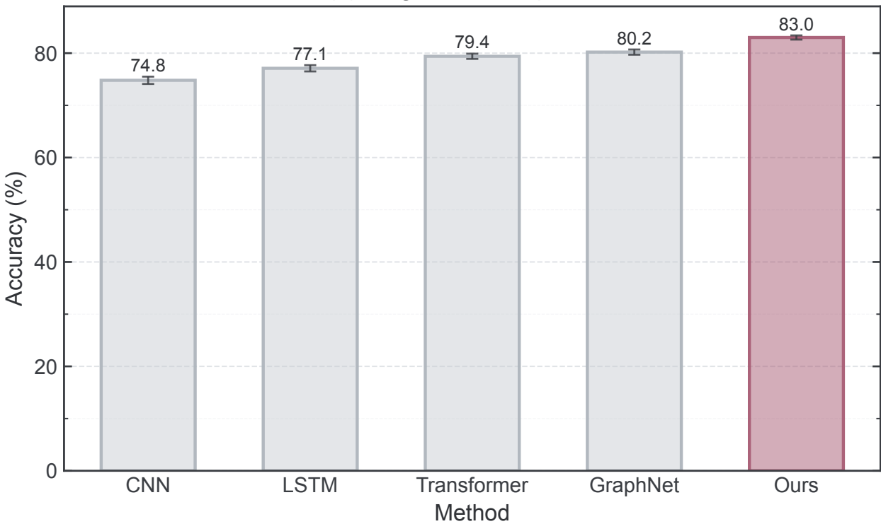
(a) Single Bar Comparison
