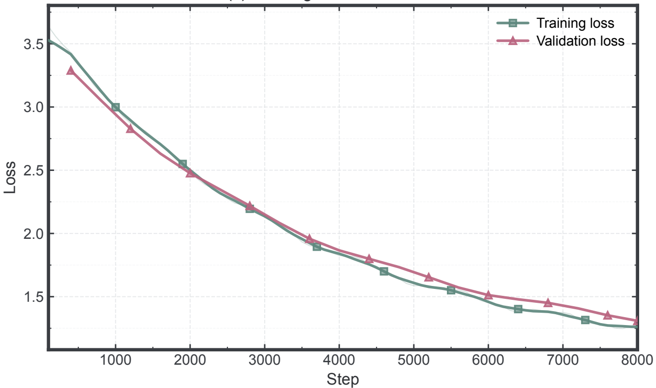
(c) Training vs. Validation Loss
