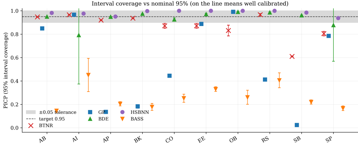
Figure 8: This figure checks whether the nominal 95% intervals contain 95% of the targets. For each model and dataset we plot the PICP (see Equation 65), with markers at the seed mean and error bars at the seed standard deviation. A dashed line marks the target of 0.95 inside a shaded tolerance band of \pm 0.05 . Points on the line are well calibrated, points below indicate overconfidence and points above indicate underconfidence. The BTNR entry is the configuration whose PICP is closest to 0.95 for each dataset. The dashed line marks the target of 0.95 inside a shaded tolerance band of \pm 0.05 .
