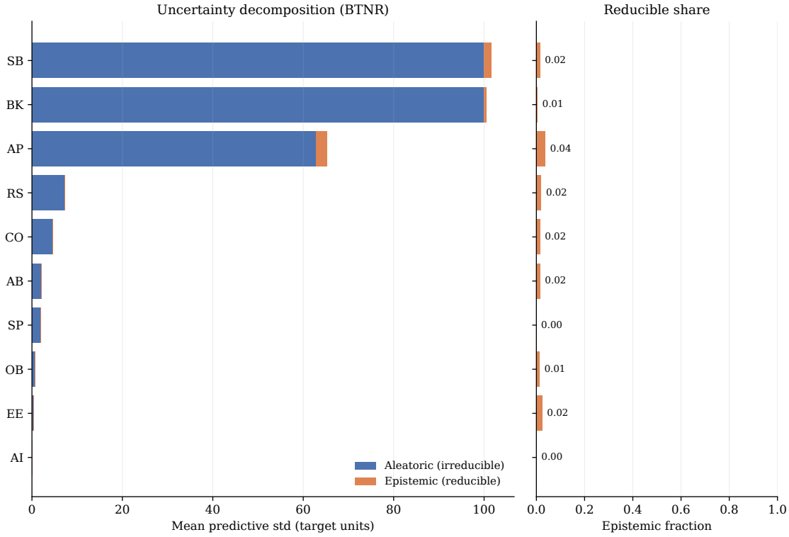
Figure 9: Uncertainty decomposition for BTNR. This figure, shows how much of the predictive uncertainty is reducible. Using the NLL best BTNR structure per dataset, the left panel stacks the mean aleatoric and epistemic standard deviations \sigma_{\text{ale}} and \sigma_{\text{epi}} in target units, with datasets sorted by their total. The right panel shows the scale free epistemic fraction \rho_{\text{epi}} (see Equation 70) defined above.
