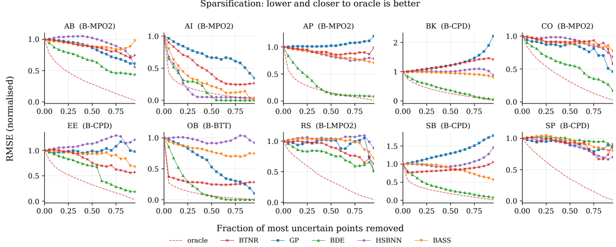
Figure 6: The plots address whether the uncertainty ranks points by error (Ilg et al., 2018). For each model we draw the normalised RMSE by uncertainty curve \widehat{\text{RMSE}}_{\text{unc}}(r) against the removal fraction r , together with the oracle curve \widehat{\text{RMSE}}_{\text{oracle}}(r) , the area between them is the AUSE (see Equation 68). A good model produces an uncertainty curve that drops quickly and stays close to the oracle, and the BTNR entry in each panel is the configuration with the lowest AUSE for that dataset.
