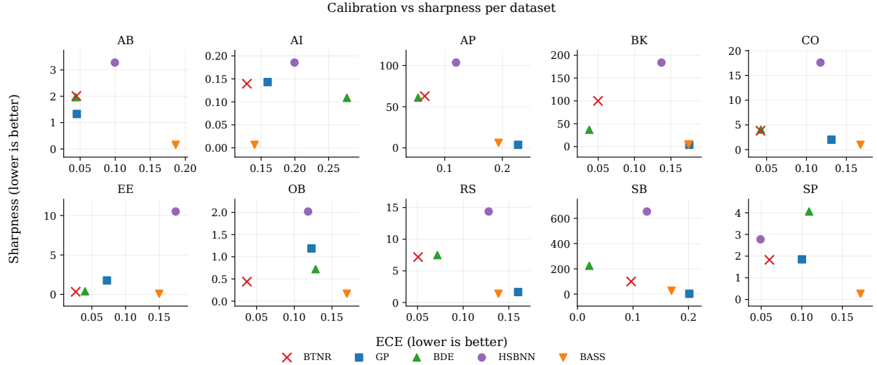
Figure 7: Each marker places a model at x = \text{ECE} (see Equation 18) and y = \text{SH} (see Equation 66), so the bottom left corner corresponds to the desirable combination of low calibration error and high confidence. The plot shows the raw pairs without normalisation, one panel per dataset. A model should be both calibrated and sharp, hence the bottom left corner (the origin) is the desirable combination of low calibration error and high confidence. For each dataset we report which tensor network structures is plotted.
