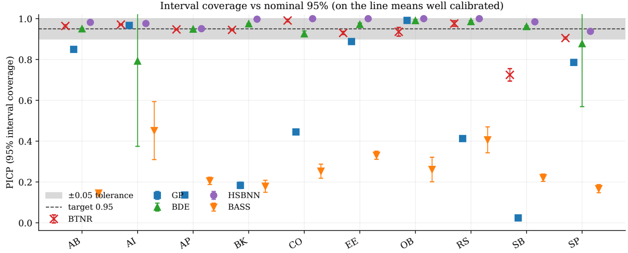
Figure 8: This figure checks whether the nominal 95% intervals contain 95% of the targets. For each model and dataset we plot the PICP (see Equation 78), with markers at the seed mean and error bars at the seed standard deviation. A dashed line marks the target of 0.95 inside a shaded tolerance band of \pm 0.05 . Points on the line are well calibrated, points below indicate overconfidence and points above indicate underconfidence. The BTNR entry is the configuration whose PICP is closest to 0.95 for each dataset with highest R^2 on the validation set . The dashed line marks the target of 0.95 inside a shaded tolerance band of \pm 0.05 .
