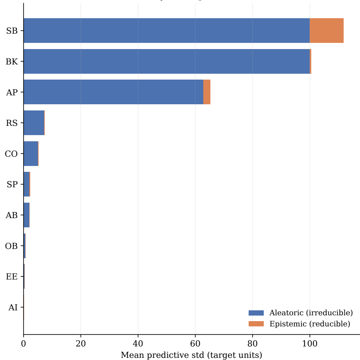
Uncertainty decomposition (BTNR)
