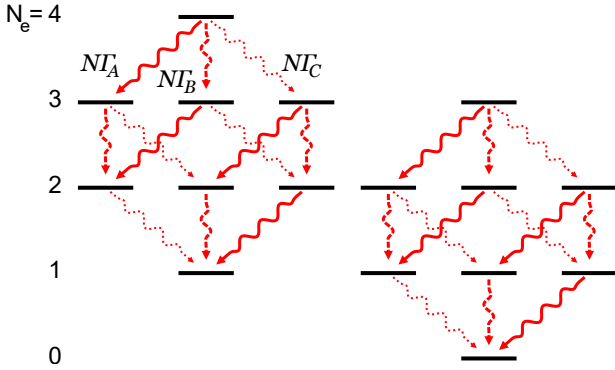
FIG. 3. Fermion emission structure for 4 atoms and 3 modes. The 16 total possible states are grouped into two sectors of 8 states each. Each sector is coupled by solid, dashed and dotted lines representing fermion emission into mode A, B and C. Connectivity in each sector is identical to a cube. For two modes, the dotted lines are eliminated, and the states fragment into 4 groups of 4 states.
