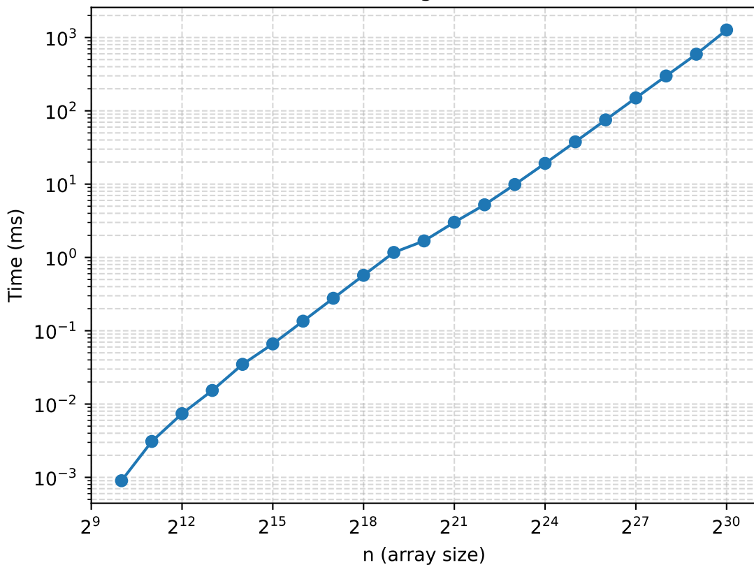
scan scaling: time vs n
