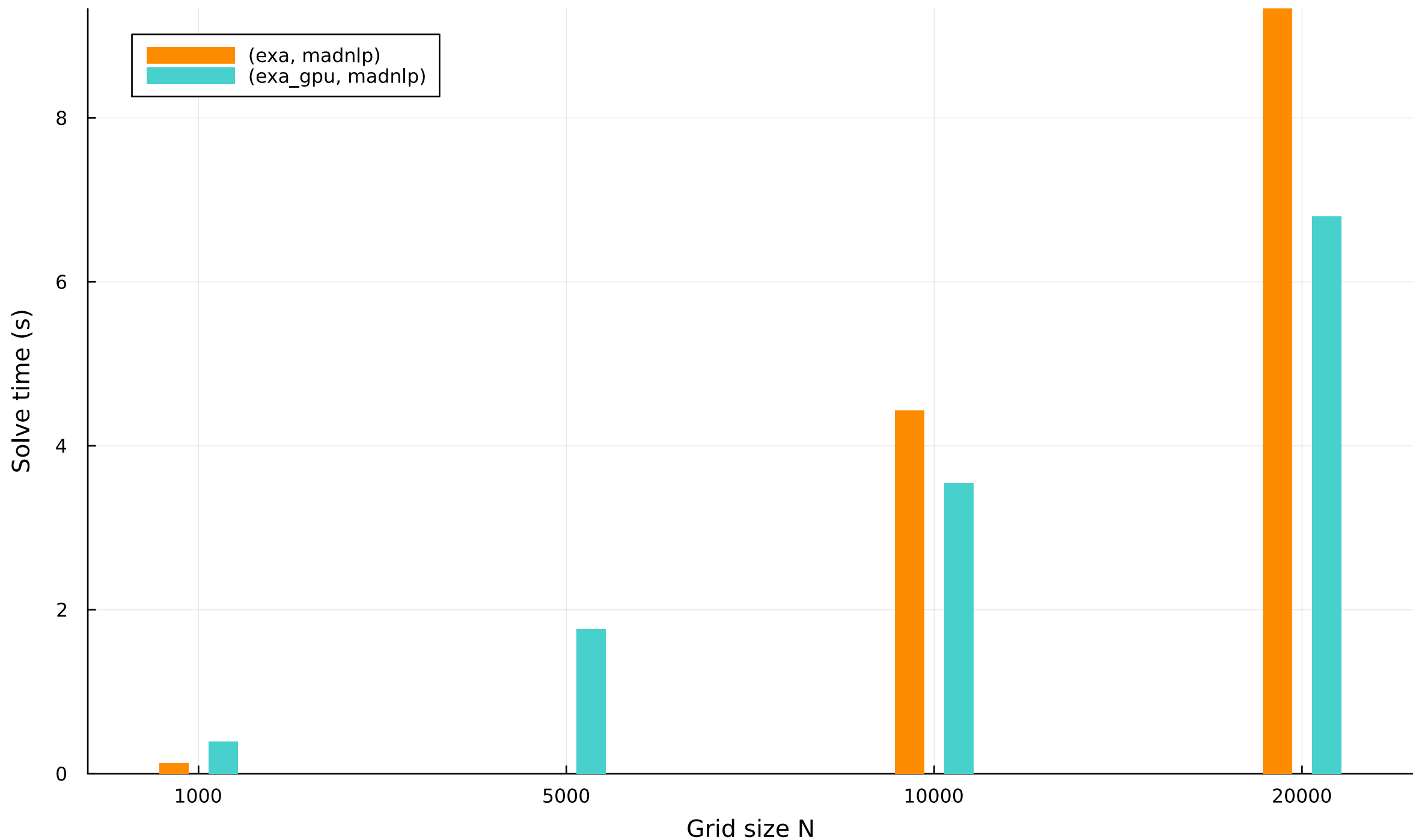
Solve time vs grid size (bar) — balanced_field
