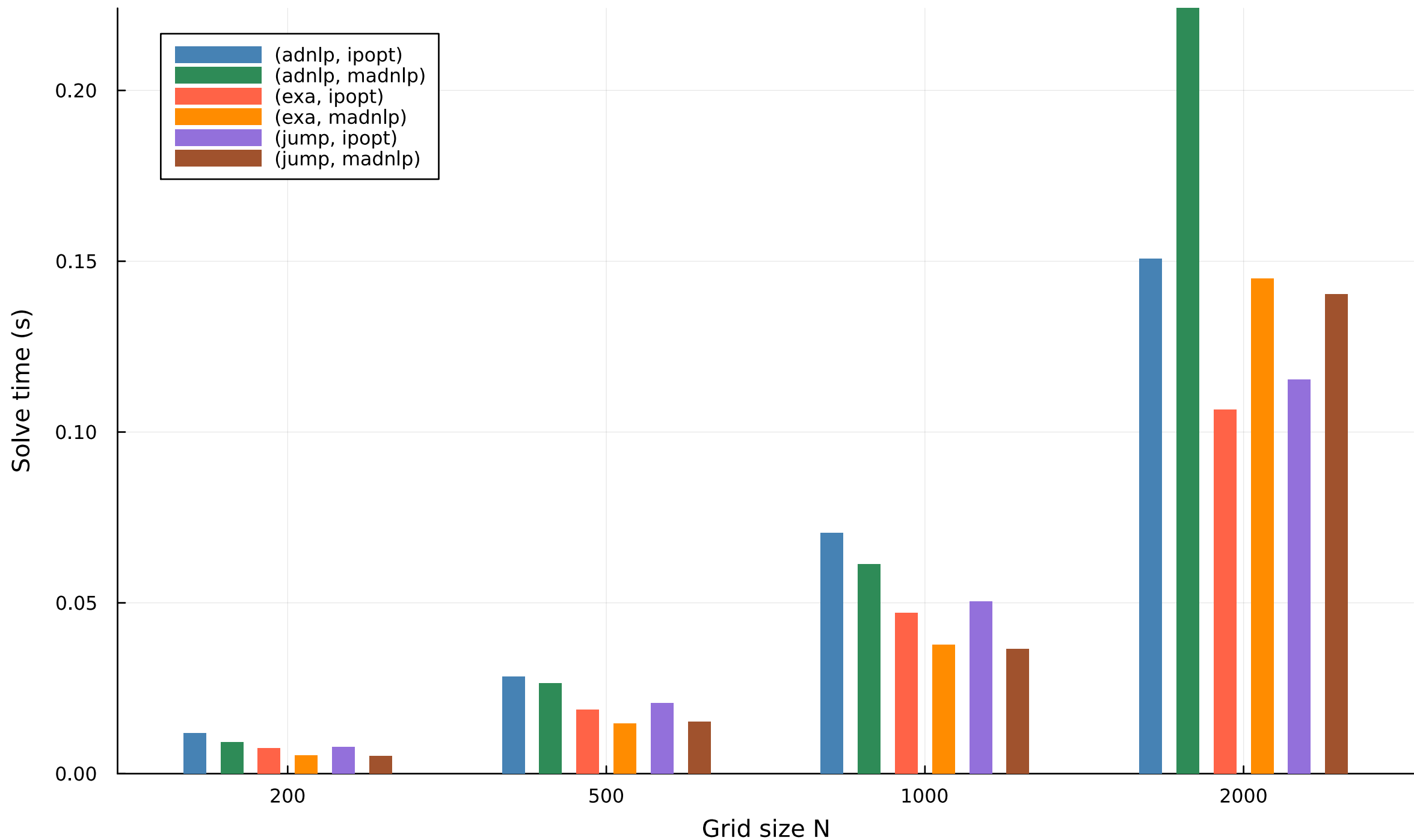
Solve time vs grid size (bar) — bryson_denham
