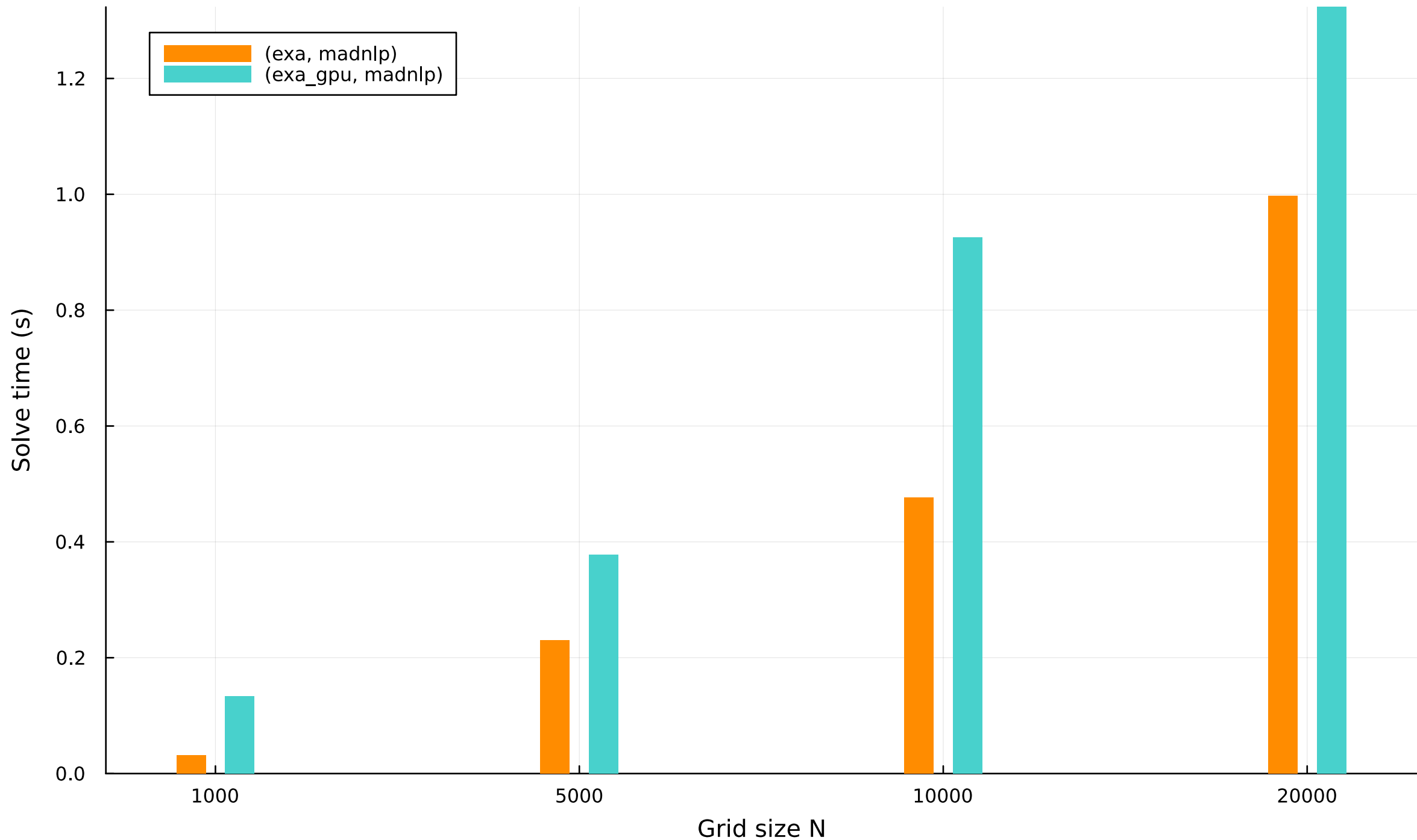
Solve time vs grid size (bar) — dielectrophoretic_particle
