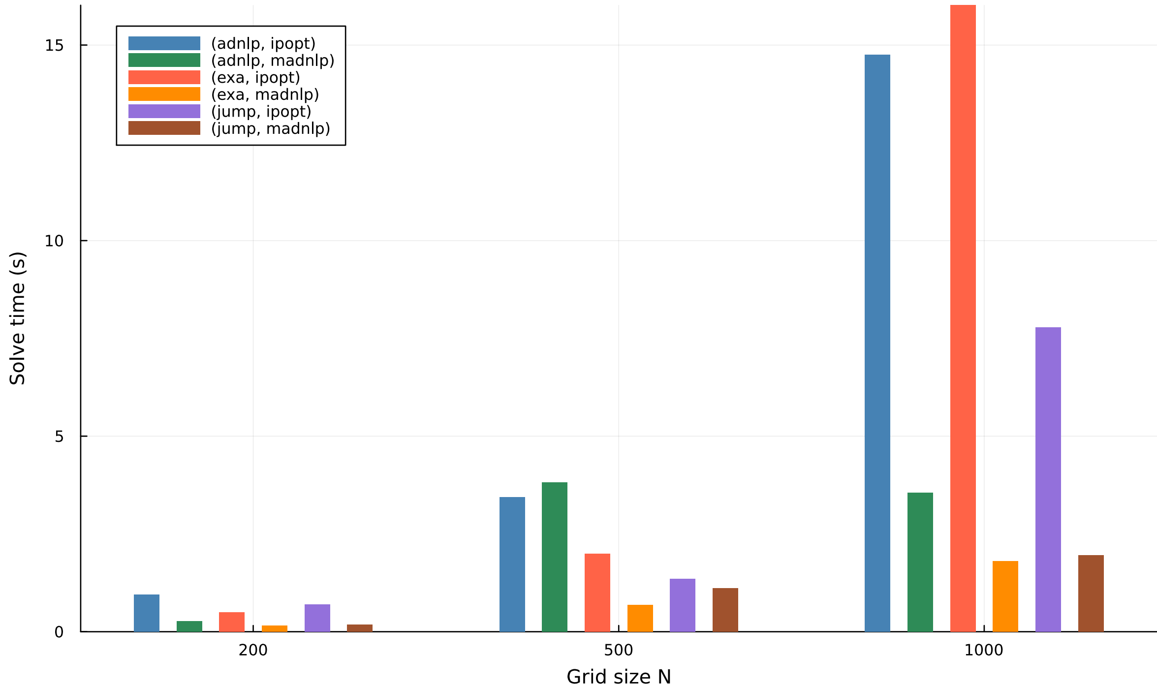
Solve time vs grid size (bar) — ducted_fan
