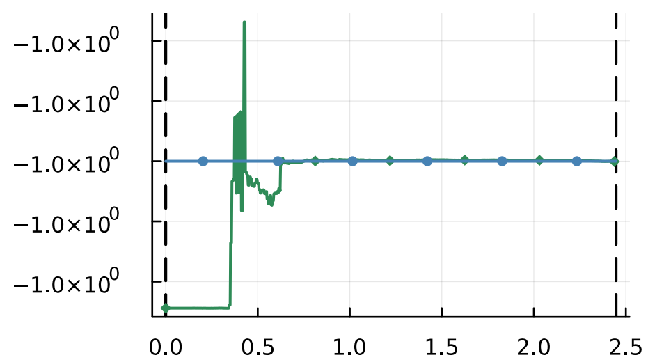
costate
