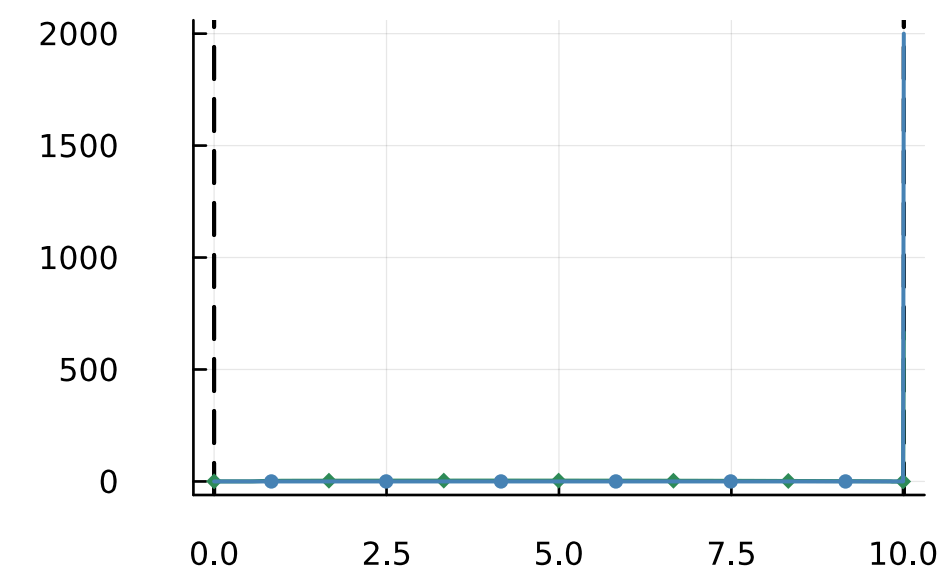
costate
