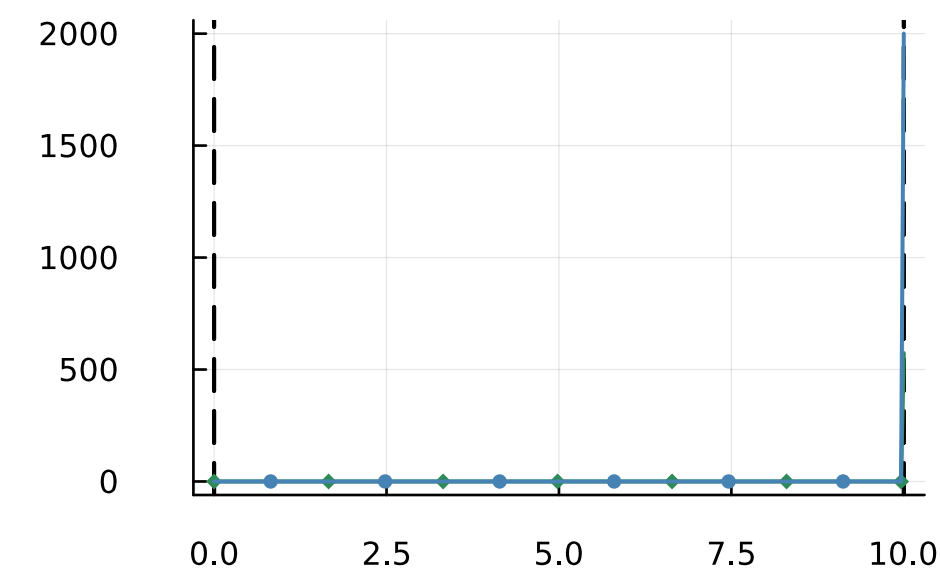
costate
