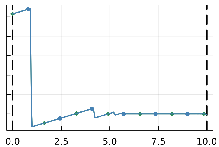
costate
