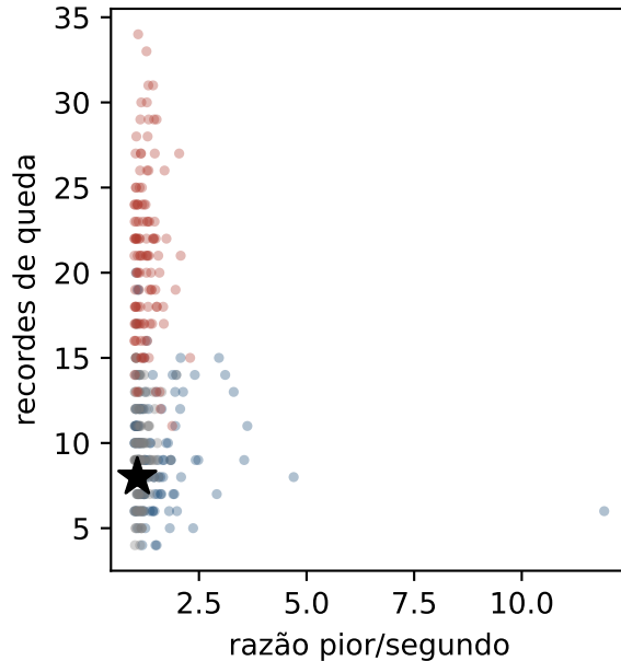
ibov
