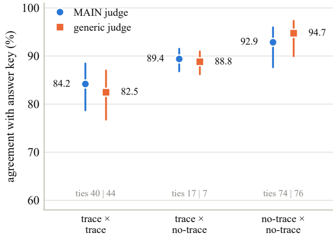
(a) all decided one-correct comparisons
