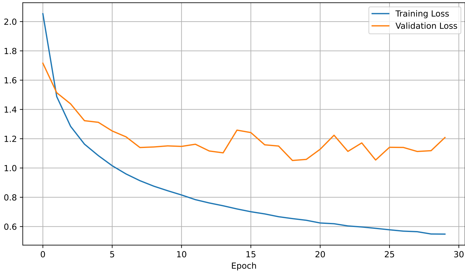
Loss across epochs
