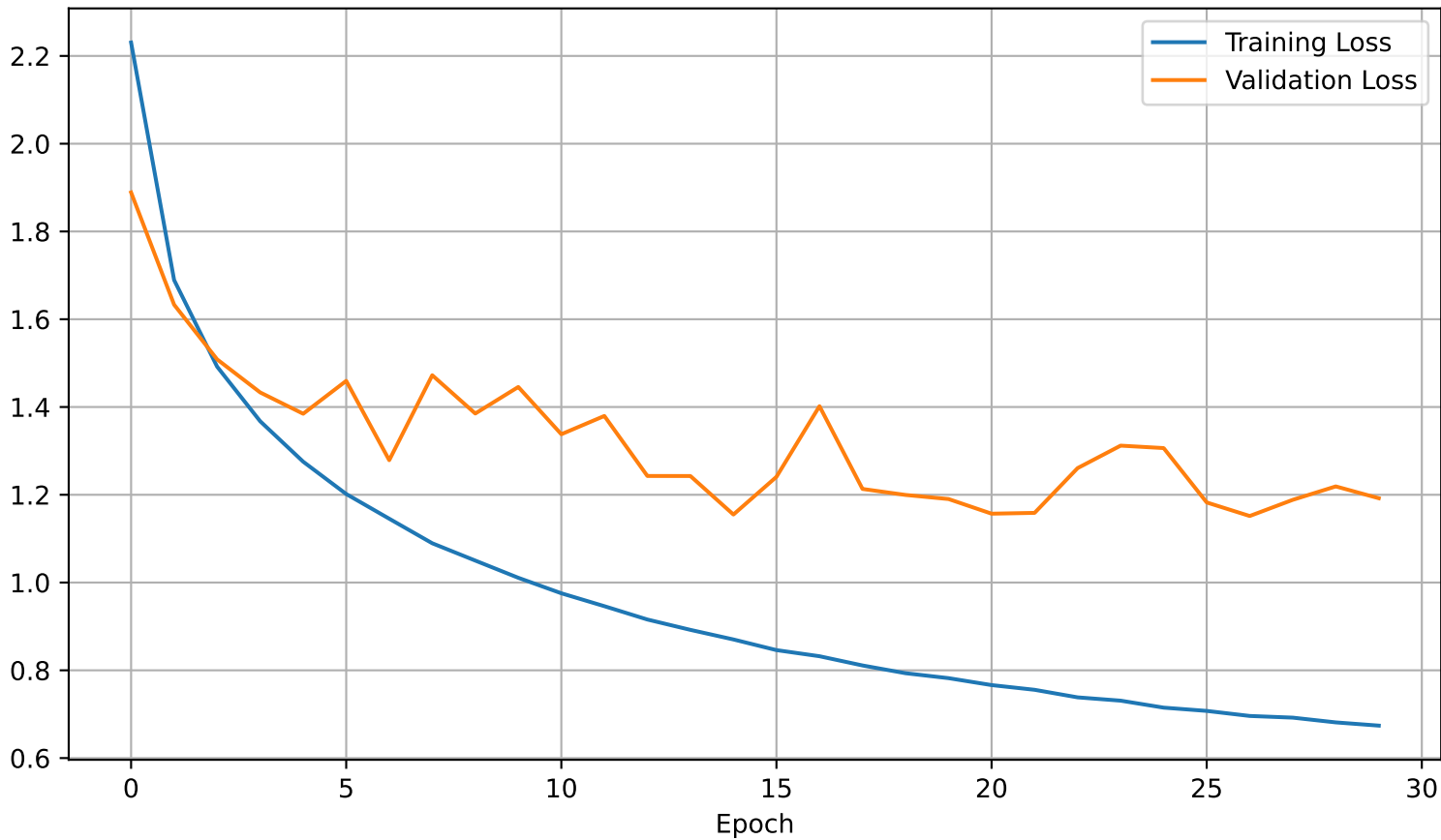
Loss across epochs
