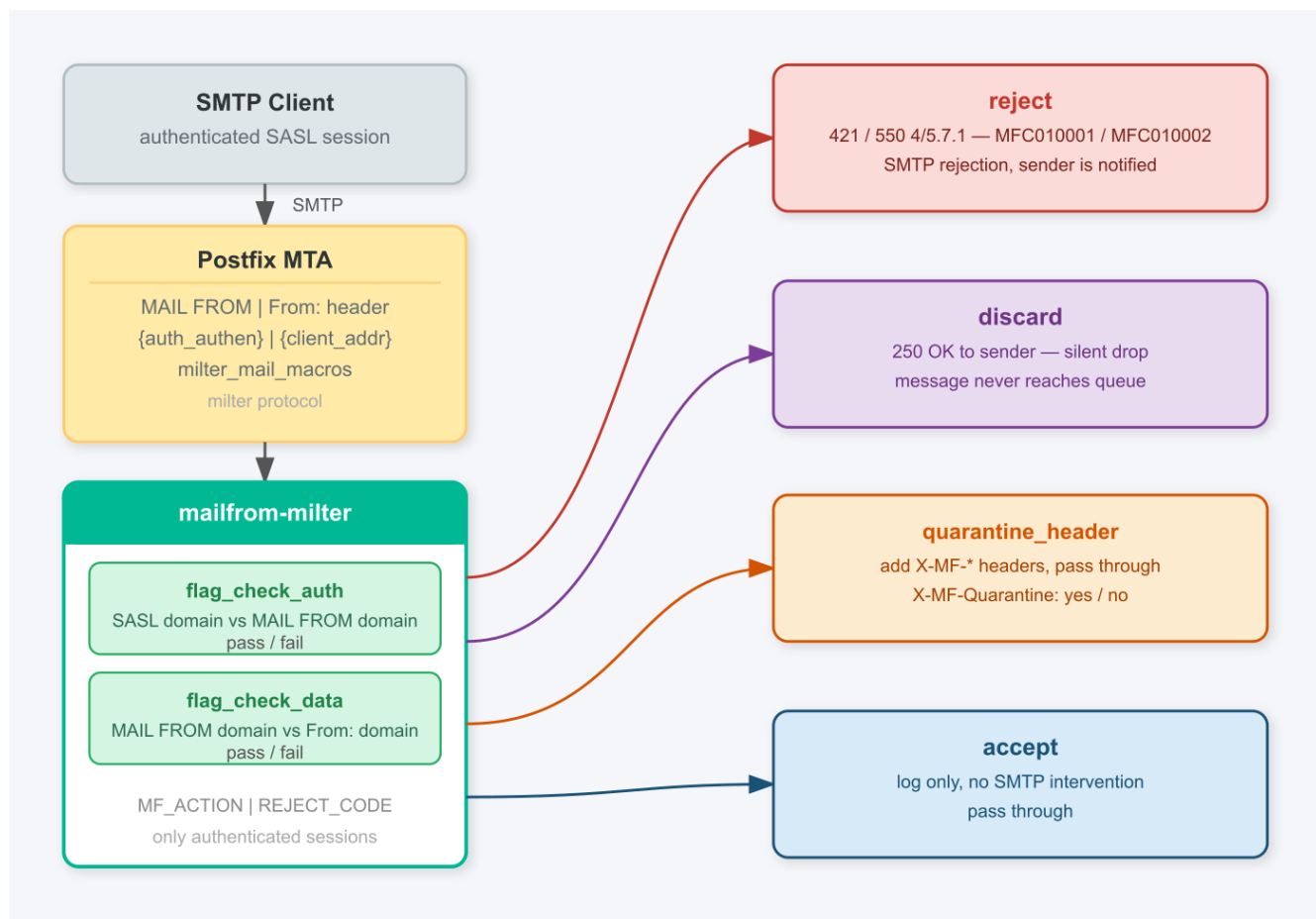
Figure 1: mailfrom-milter architecture
