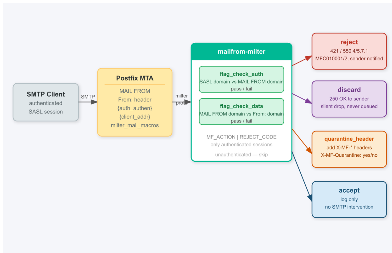
Figure 1: mailfrom-milter architecture
